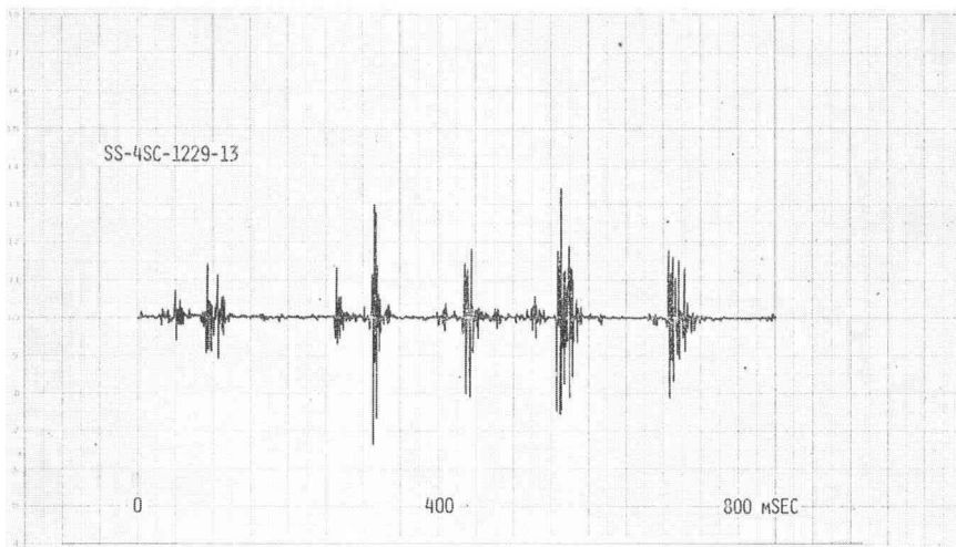
Fig. 6. Typical acoustic emission signals immediately after blasting.
