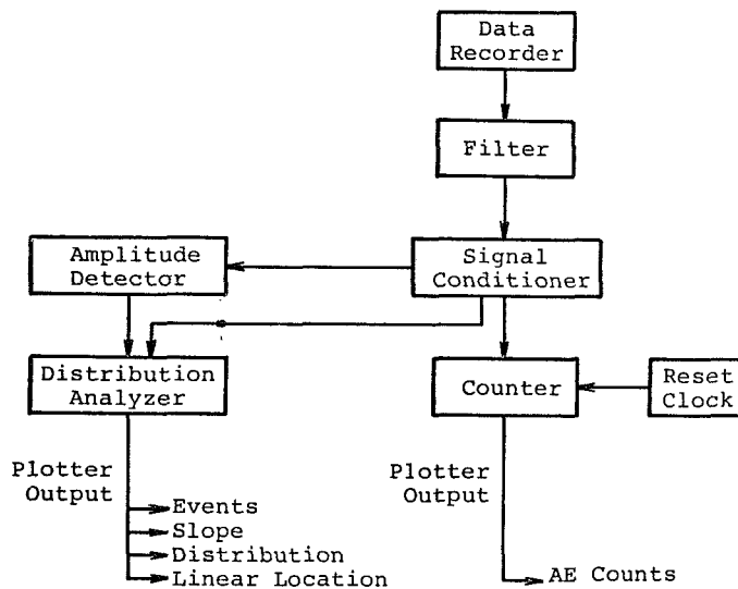
Fig. 4. Acoustic emission analyzing facility.
