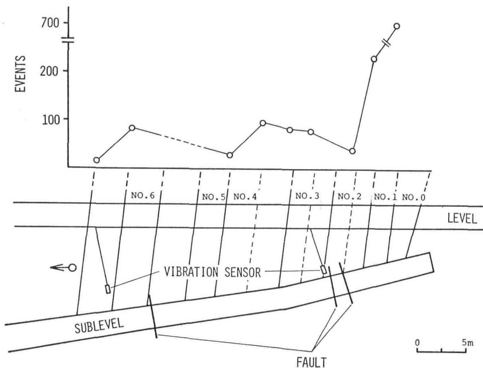
Fig. 13. Variation of accumulated events per unit time with advance of working face in hydraulic mining.
