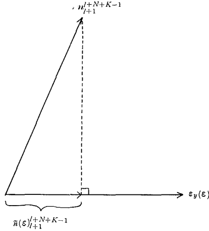
Fig. 2. Orthogonal projection of \mathbf{n}_{l+1}^{l+N+K-1} on \boldsymbol{\varepsilon}_y(\varepsilon) .
