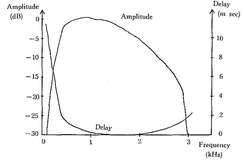
Fig. 4. Frequency characteristic of Channel 2.
