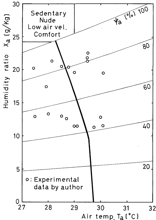
Fig. 6. Verification of the present comfort line.
