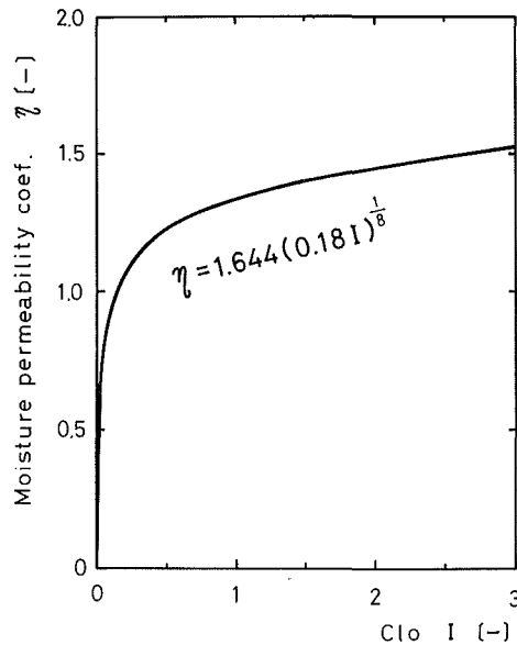
Fig. 5. Relation between moisture permeability coefficient and clo value 10) .
