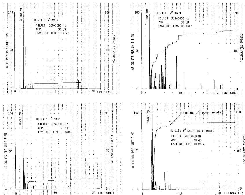
Fig. 6. Acoustic emission activity after blasting in drive.
