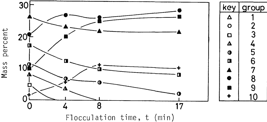
Fig. 3. Time variation of mass percent of flocs (Experimental run 6)
