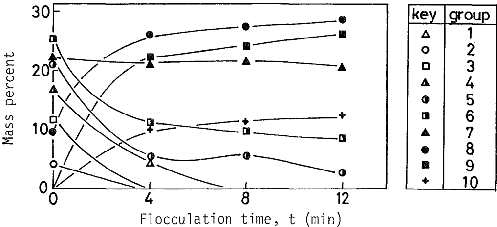
Fig. 1. Time variation of mass percent of flocs (Experimental run 3)
