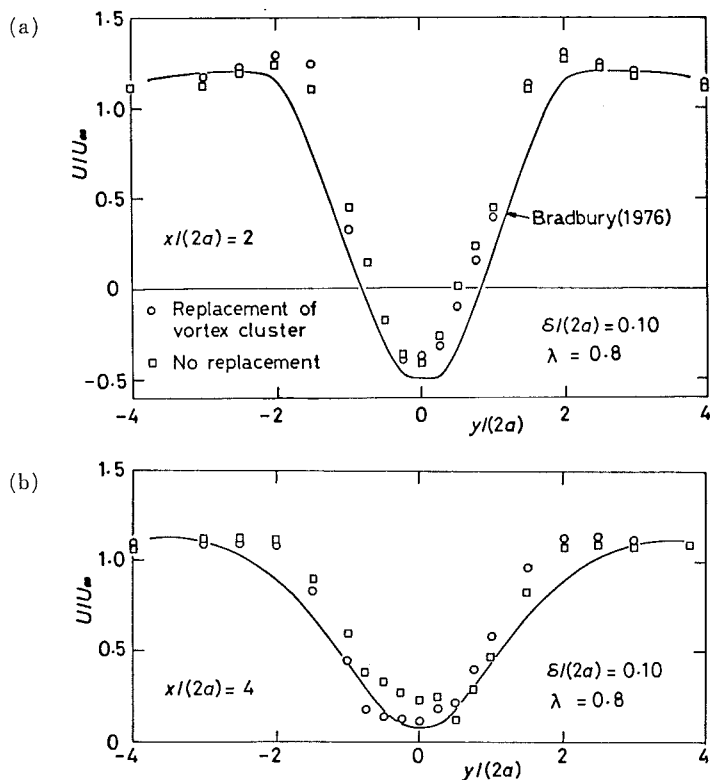
Fig. 5. Distribution of time-averaged longitudinal velocity component in near wake.
