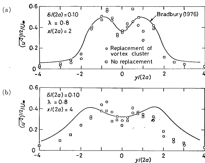
Fig. 6. Distribution of root-mean-square value of fluctuating longitudinal velocity component.
