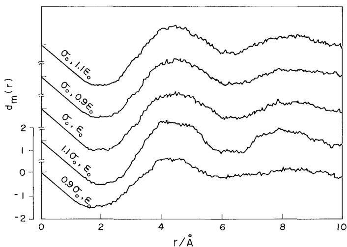
Fig. 6. Comparison of calculated d_m(R) .
