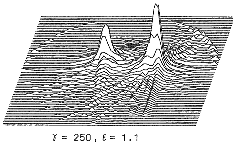
Fig. 5 Best ESR image with \gamma=250 and \epsilon=1.1 .
