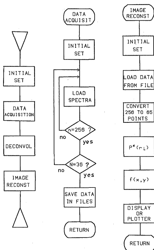
Fig. 1 Flow chart of programs for controlling ESR apparatus, data acquisition, deconvolution and image reconstruction.
