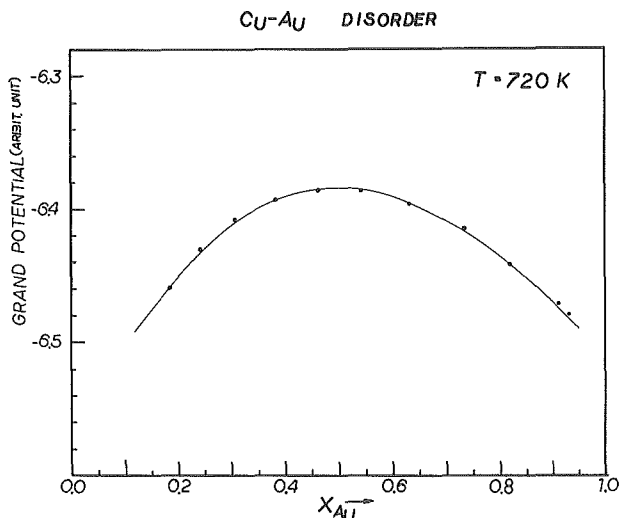
Fig. 2 Concentration dependency of Grand potential in arbitrary unit of disorder phase at 720 K. Horizontal axis indicates atomic concentration of Au.
