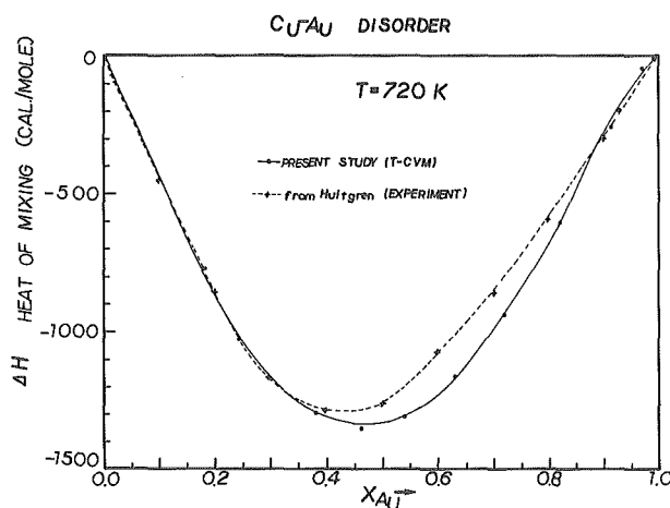
Fig. 4 Concentration dependency of Heat of Mixing of disorder phase. Present study is drawn by solid line and the experimental results quoted from Hultgren 17) are indicated by broken line.
