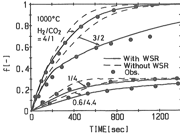
Fig. 5 Comparison of the observed fractional reduction with the calculated by considering water-gas shift reaction. ( H_2-CO_2 , 1000°C, 5g)
