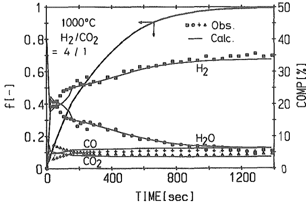
Fig. 8 The fractional reduction and utilization of H_2 and CO . ( H_2/CO_2=1/4 , 1000^\circ C , 5g)
