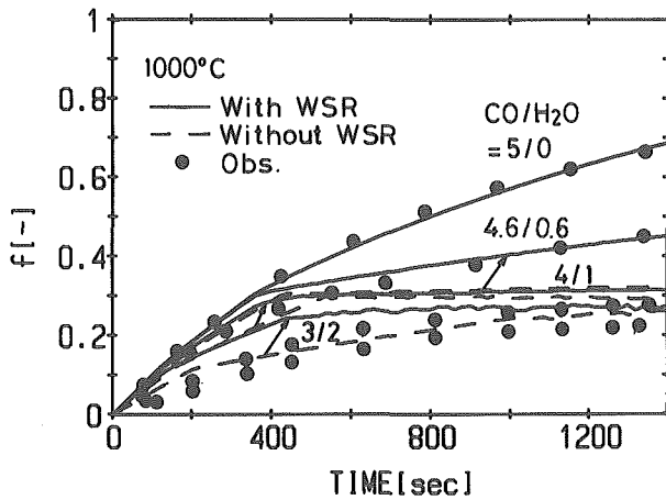
Fig. 6 Comparison of the observed fractional reduction with the calculated by considering water-gas shift reaction. ( CO-H_2O , 1000°C, 5g)
