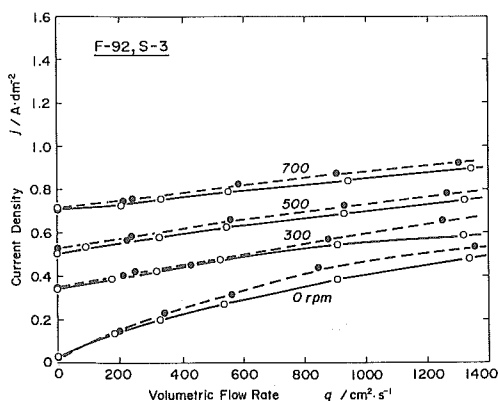
Fig. 10 Comparison of diffusion limiting currents at different numbers of fins ( l_h = 2 mm, l_g = 3 mm) on the S-3 in F-92. Solid line: four fins and broken line: eight fins.
