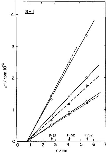
Fig. 13 Relation between the reciprocal of the equivalent rotational speed and rotor radius on the S-1 surface in the three cells. l_g (mm): \circ=3 , \bullet=2 .
