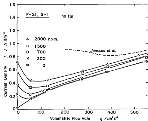
Fig. 4 Diffusion limiting current density as a function of the volumetric flow rate per unit height of gap at various rotational speeds on the S-1 surface in F-21 cell without fins.
