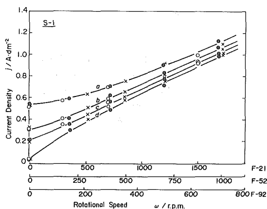
Fig. 12 Best fitting curves of the diffusion limiting current density on the S-1 surface ( l_g=3 mm) of the three cells: \circ =F-21, \times =F-52, and \bullet =F-92. Volumetric flow rates per unit height of gap for F-21, F-52, and F-92 are: a=361, 722, and 1110 \text{cm}^2\cdot\text{s}^{-1} , b=167, 361, and 556 \text{cm}^2\cdot\text{s}^{-1} , c=111, 194, and 278 \text{cm}^2\cdot\text{s}^{-1} , d=0, 0, and 0 \text{cm}^2\cdot\text{s}^{-1} .
