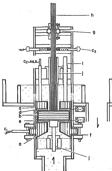
Fig. 1 Test cell: (a) stator, (b) rotor, ( c_1 , c_2 , c_3 ) lead wire, (d) acrylic fin, (e) acrylic spacer, (f) silicone rubber packing, (g) ball bearing, (h) rotating shaft (brass), (i) fixing rod, and (j) pillow block.
