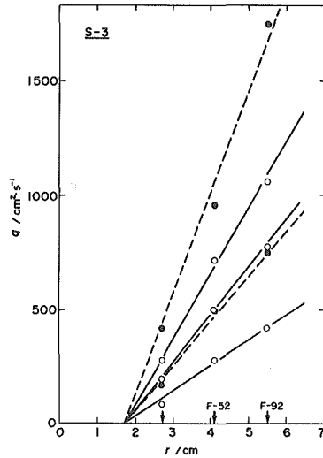
Fig. 16 Relation between the equivalent volumetric flow rate per unit height of gap and rotor radius on the S-3 surface in the three cells. l_g (mm): \circ=3 , \bullet=2 .
