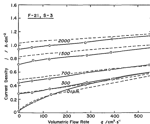
Fig. 7 Diffusion limiting current density as a function of the volumetric flow rate per unit height of gap at various rotational speeds on the S-3 surface in F-21 cell with fins. Solid line: l_g = 3 mm, broken line: l_g = 2 mm. Fins ( f_h = 2 mm, four pieces).
