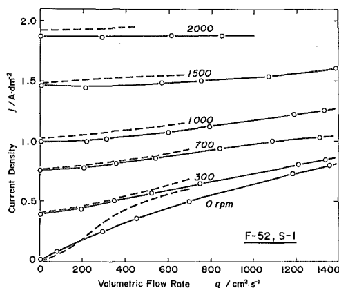
Fig. 8 Comparison of diffusion limiting currents at different height of fins on the S-1 in F-52. Solid line: l_g = 3 mm, f_h = 2 mm, and broken line: l_g = 6 mm, f_h = 5 mm.
