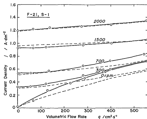
Fig. 6 Diffusion limiting current density as a function of the volumetric flow rate per unit height of gap at various rotational speeds on the S-1 surface in the F-21 cell with fins. Solid line: l_g = 3 mm, broken line: l_g = 2 mm. Fins ( f_h = 2 mm, four pieces).
