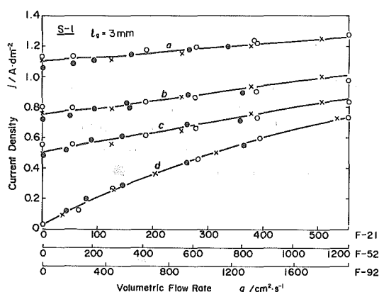
Fig. 11 Best fitting curves of the diffusion limiting current density on the S-1 surface ( l_g=3 mm) of the three cells: \circ =F-21, \times =F-52, and \bullet =F-92. Rotational speeds for F-21, F-52, and F-92 are: a-1900, 1100, and 800 rpm, b=1250, 700, and 500 rpm, c=750, 400, and 300 rpm, d=0, 0, and 0 rpm.
