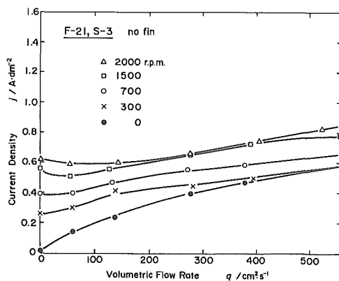
Fig. 5 Diffusion limiting current density as a function of the volumetric flow rate per unit height of gap at various rotational speeds on the S-3 surface in F-21 cell without fins.
