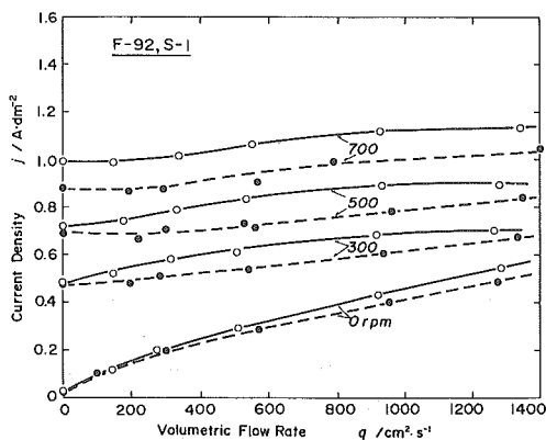
Fig. 9 Comparison of diffusion limiting currents at different numbers of fins ( l_h = 2 mm, l_g = 3 mm) on the S-1 in F-92. Solid line: four fins and broken line: eight fins.
