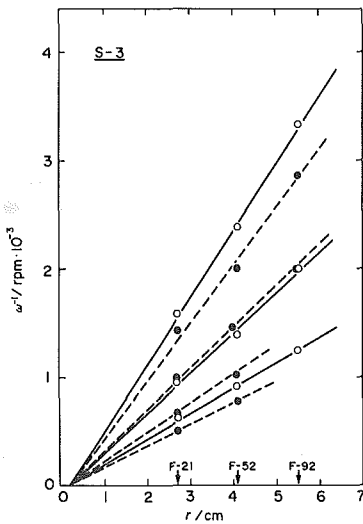
Fig. 15 Relation between the reciprocal of the equivalent rotational speed and rotor radius on the S-3 surface in the three cells. l_g (mm): \circ=3 , \bullet=2 .
