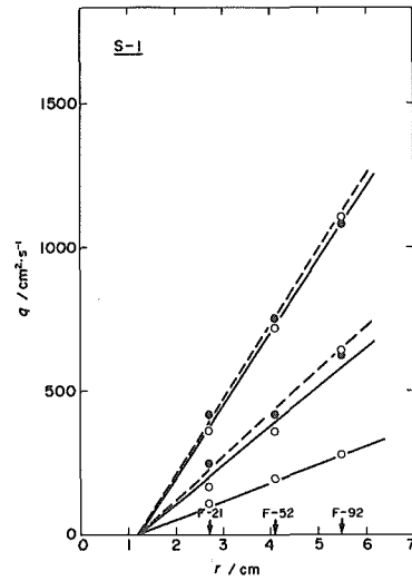
Fig. 14 Relation between the equivalent volumetric flow rate per unit height of gap and rotor radius on the S-1 surface in the three cells. l_g (mm): \circ=3 , \bullet=2 .
