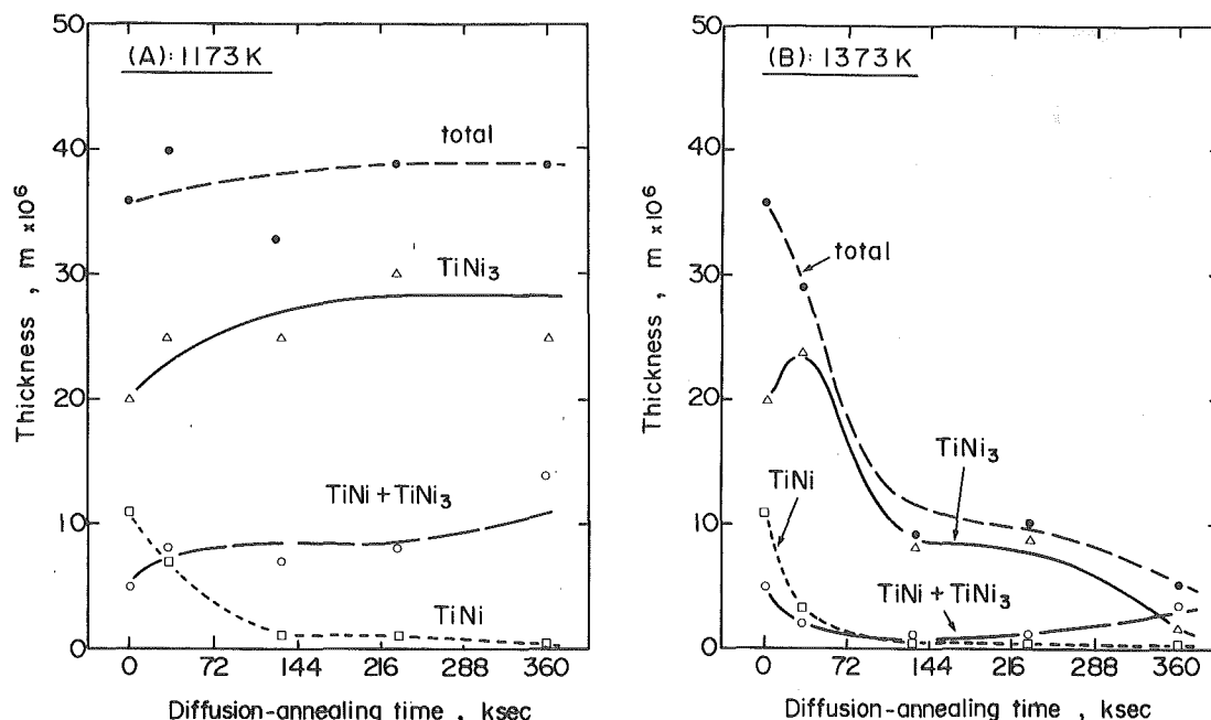
Figure 7 Changes in the layer thicknesses of the \text{TiNi}_3 , \text{TiNi} , a mixture of \text{TiNi} and \text{TiNi}_3 , and total of them with diffusion-annealing times. A: 1173 K and B: 1373 K.
