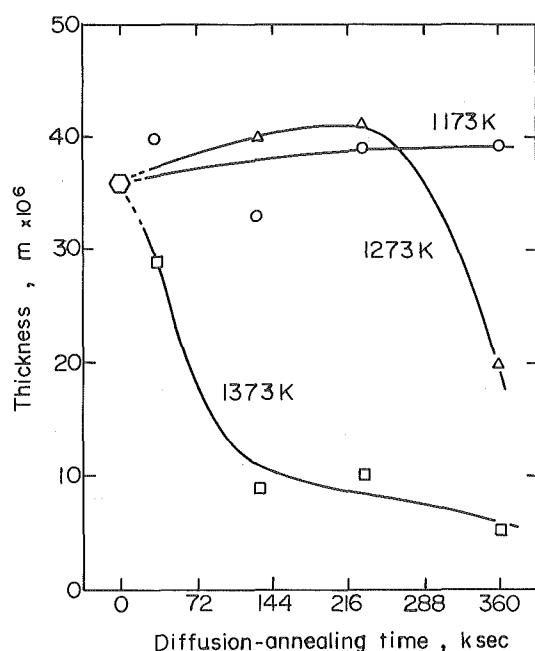
Figure 9 Changes in the total thickness of the intermetallic compounds with the diffusion-annealing times at 1173, 1273, and 1373 K.
