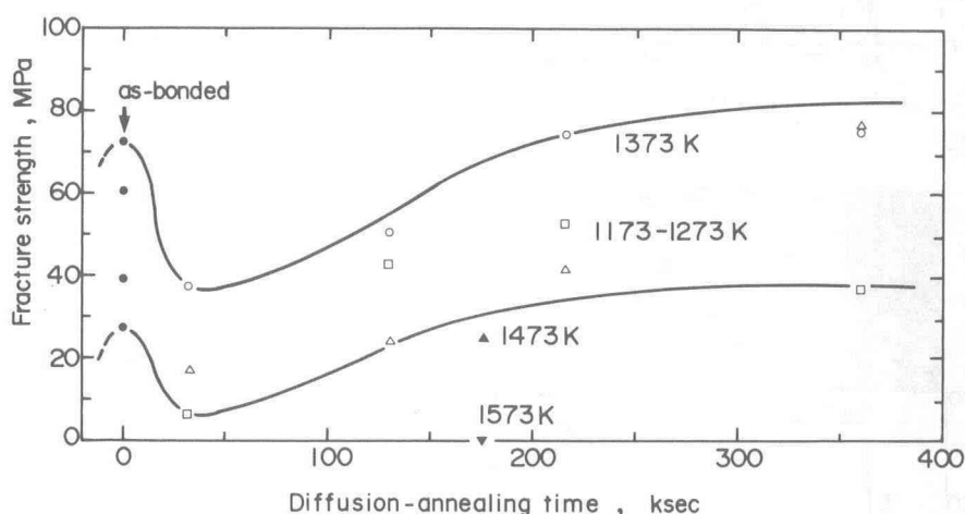
Figure 6 Variations of the fracture strengths with diffusion-annealing times at temperatures between 1173 and 1573 K, where the bonding has been made at 1423 K for 3.6 ksec.
