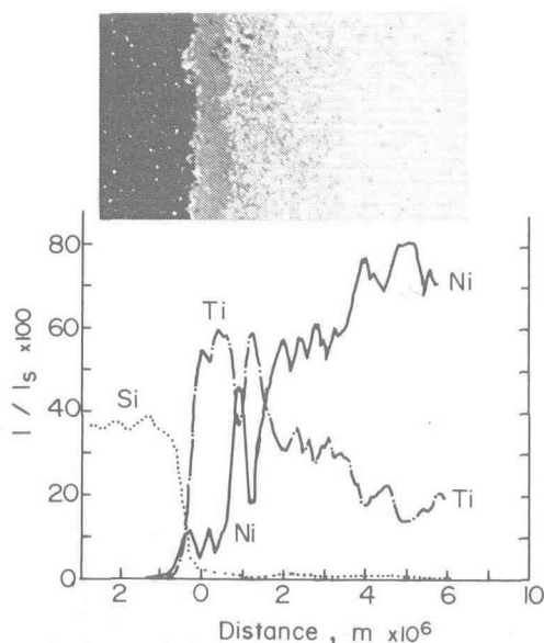
Figure 8 Enlarged microstructures of the ceramic-filler metal interface and concentration profiles of Ti, Si, and Ni.
