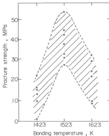
Figure 2 Temperature dependences of the fracture strengths of the bondings made for 1.8 ksec at temperatures of 1423, 1523, and 1623 K.
