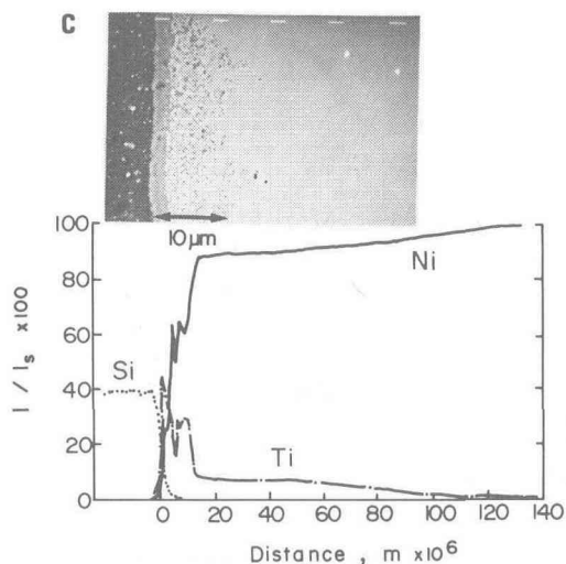
Figure 3 Microstructures and line analyses of Ti, Si, and Ni across the ceramic/metal bondings made at 1423 K for various times. A : 1.8 ksec, B : 3.6 ksec, and C : 18.0 ksec.
