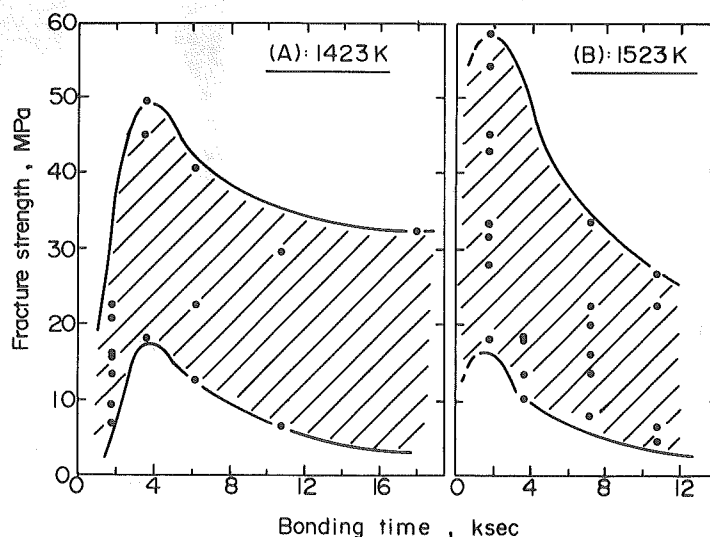
Figure 1 Changes in the fracture strengths with bonding times. (A) 1423 K, (B) 1523 K.
