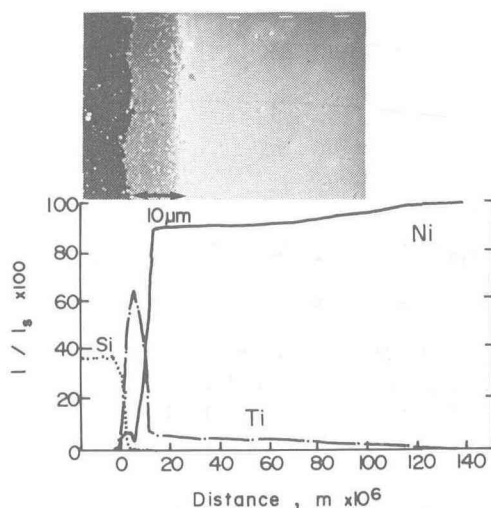
Figure 4 Microstructure and line analyses of Ti, Si, and Ni across the ceramic/metal bonding made at 1523 K for 1.8 ksec.
