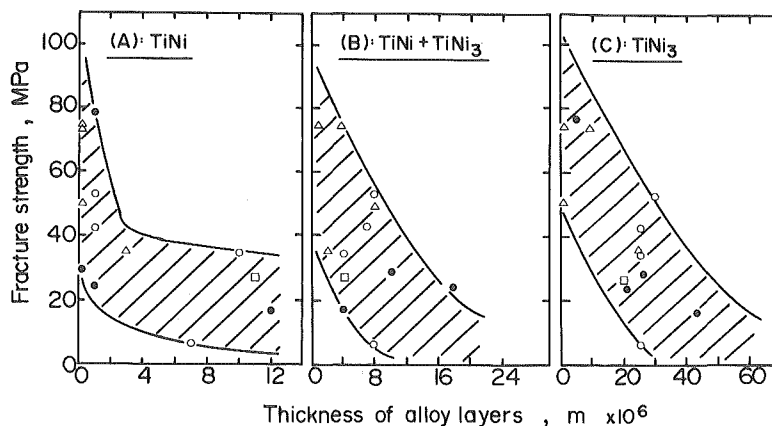
Figure 10 Changes in the fracture strengths with the layer thicknesses of (A) TiNi, (B) a mixture of TiNi and TiNi 3 , (C) TiNi 3 .
