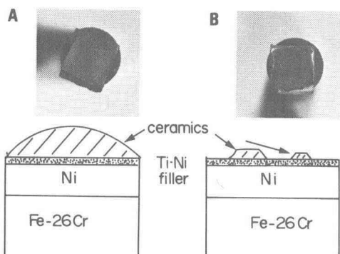
Figure 5 Morphologies of the fractured surfaces of the bondings and their schematic structures. A: failure through ceramics and B: interfacial failure.
