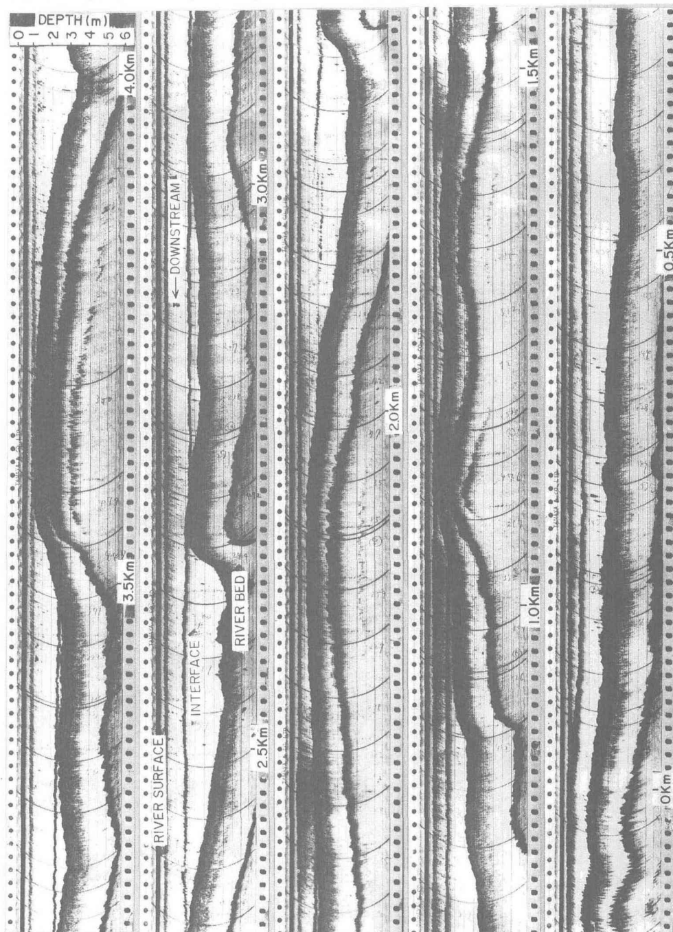
Fig. 3 A longitudinal profile of the salt wedge at the Shiribetsu River (July 23, 1977).
