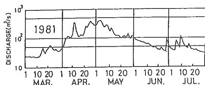
Fig. 10 A change of the river discharge of the Shiribetsu River (March ~July, 1981).
