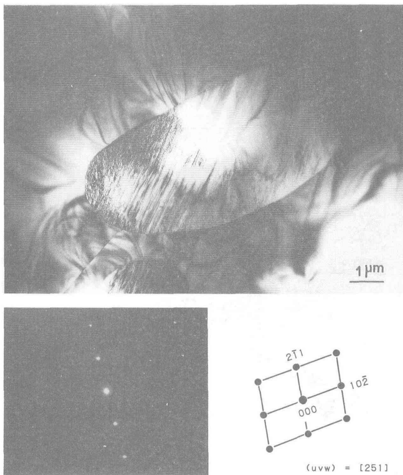
Fig. 7 Bright field electron micrograph near the [251]_{1:5} beam direction after aging 30 min at 850^\circ\text{C} .
