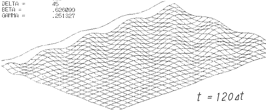
Fig. 7 Development of reflection The incident angle is 45^\circ
