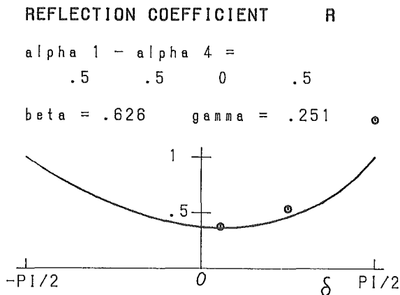
Fig. 4 Reflection coefficient Scheme II-1 \beta = .625 \quad \gamma = .251
