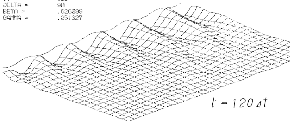
Fig. 8 Development of reflection The incident angle is 90^\circ
