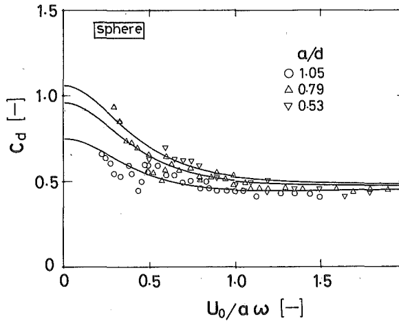
Fig. 3 Variation of drag co-efficient with U_0/a\omega
