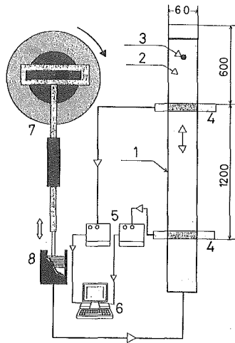
Fig. 4 Schematic diagram of experimental apparatus. 1. test section; 2. tap water; 3. test particle; 4. sensor; 5. sensor amplifier; 6. digital recorder; 7. Scotch-York; 8. piston and cylinder
