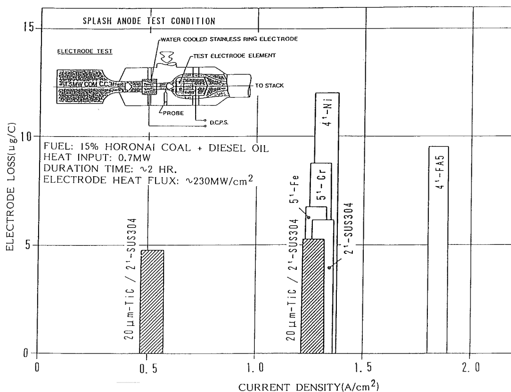
Fig. 12 The average wear of TiC electrodes with a current density of 1.3 A/cm 2 as compared with the various pure metal and alloy electrodes.
