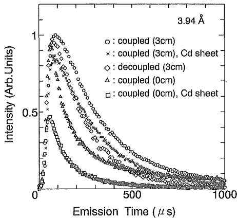
Fig. 2 Comparison of the Pulse shapes of cold neutrons.
