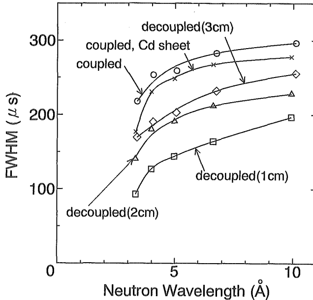
Fig. 10 Premoderator thickness dependence of the pulse widths.
