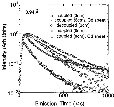
Fig. 4 Semi-logarithmic plots of the pulse shapes.
