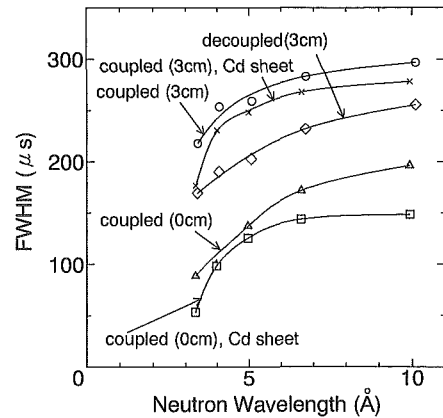
Fig. 3 Pulse widths from the two different systems.
