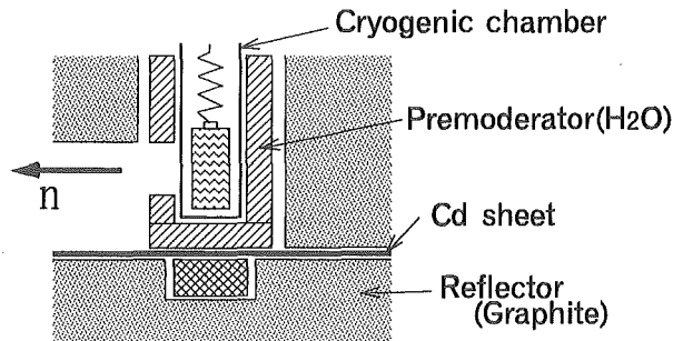
Fig. 1 Experimental set-up of target-moderator-reflector systems.
