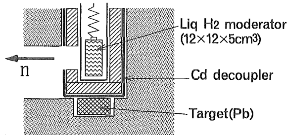
(a) Decoupled composite moderator system
