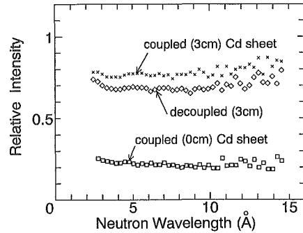
Fig. 5 Relative values of time-integrated intensities from the coupled composite moderator with Cd sheet and from the decoupled one.
