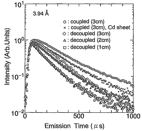
Fig. 9 Semi-logarithmic plot of premoderator thickness dependence of the pulse shapes.
