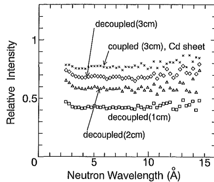
Fig. 7 Relative value of time-integrated intensities from the decoupled composite moderator with various premoderator thickness.
