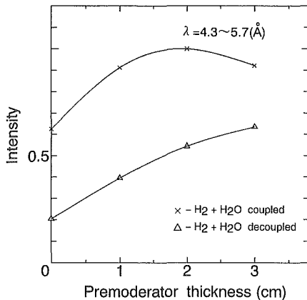
Fig. 6 Cold neutron intensity from the decoupled composite moderator as a function of the premoderator thickness.
