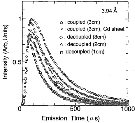
Fig. 8 Premoderator thickness dependence of the pulse shapes.
