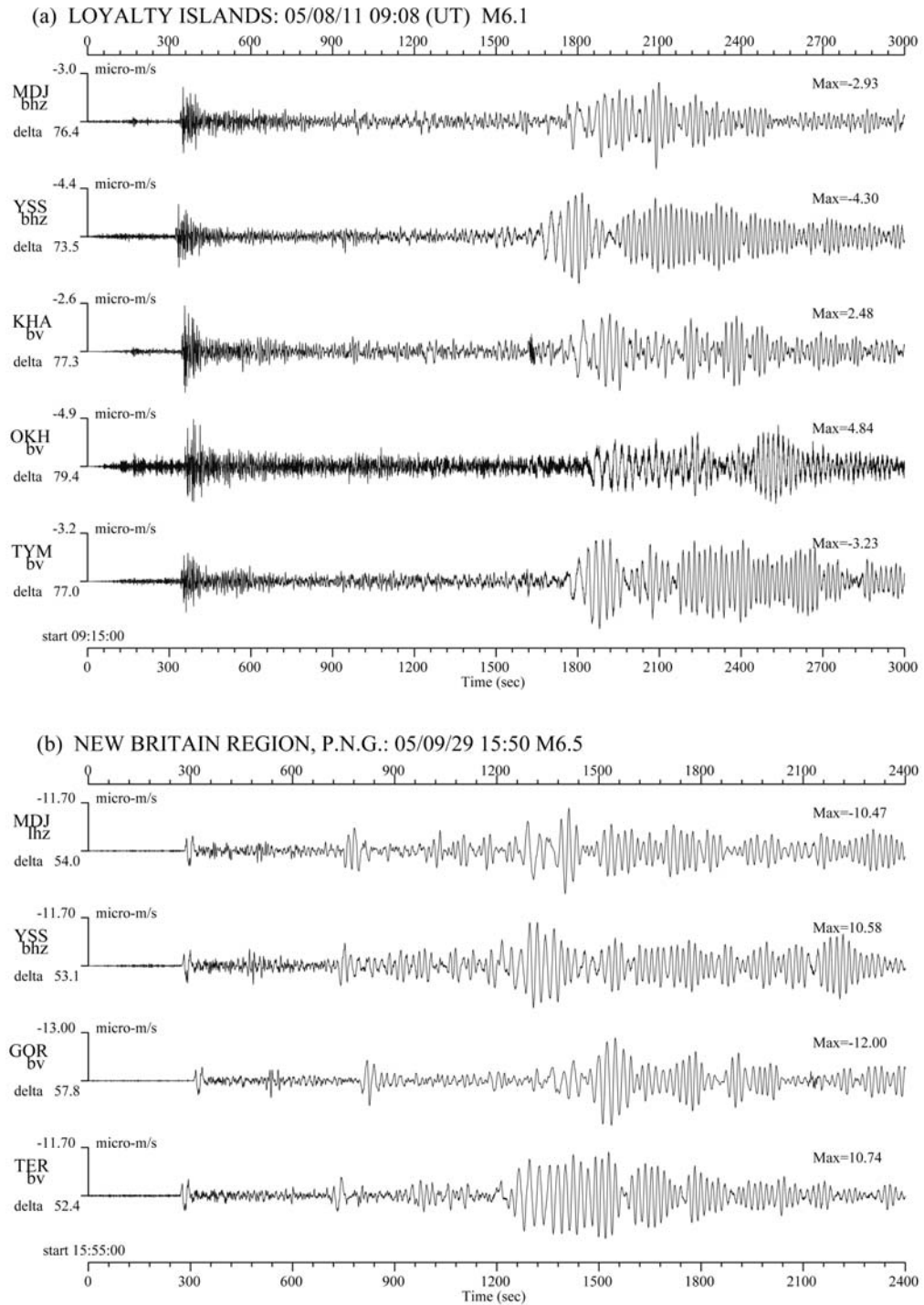
Fig. 3. Comparison of seismic waves observed at our broadband seismic stations with those at the IRIS seismic stations MDJ and YSS; (a) shows seismograms of the Mw6.1 Loyalty Islands earthquake on August 11, 2005, and (b) those of the Mw6.5 New Britain Region earthquake on September 29, 2005.
