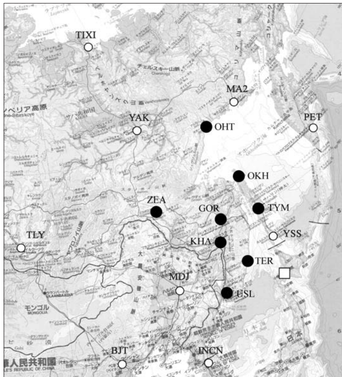
Fig. 1. A distribution of the broadband seismic stations located in Far-eastern Russia. Solid and open circles denote the seismic stations operated in this study and the IRIS seismic stations, respectively. Three-letter station code is attached, which is listed on Table 1. An open square indicates Institute of Seismology and Volcanology, Hokkaido University.
