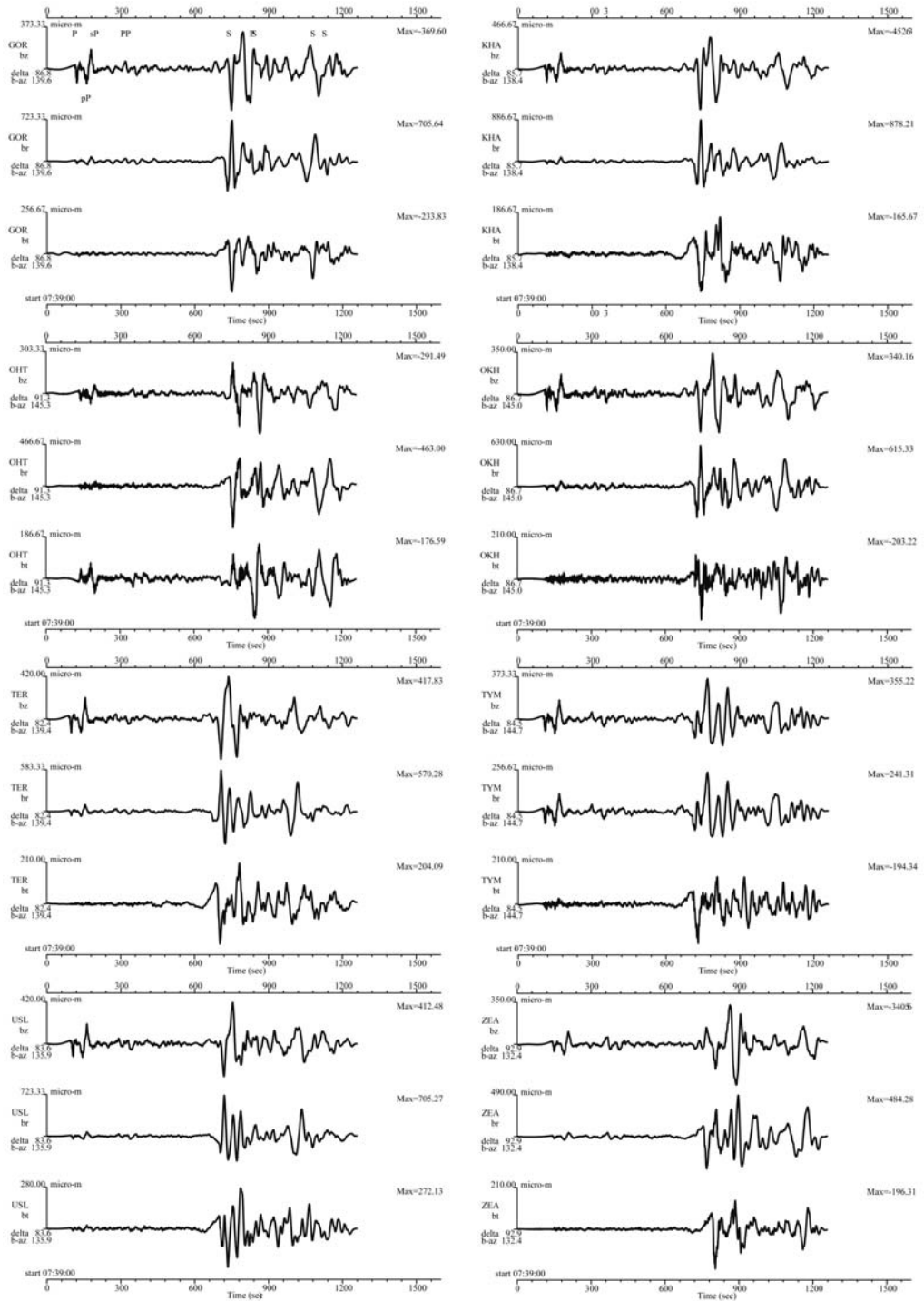
Fig. 4. Seismograms recorded at each station by the Mw 7.7 earthquake occurred at Fuji Islands on 07h28m, December 9, 2007.
