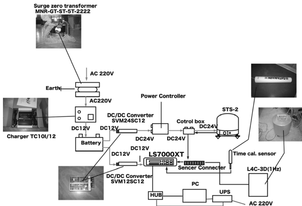
Fig. 2. Illustration of the instrumentation at each seismic station.
