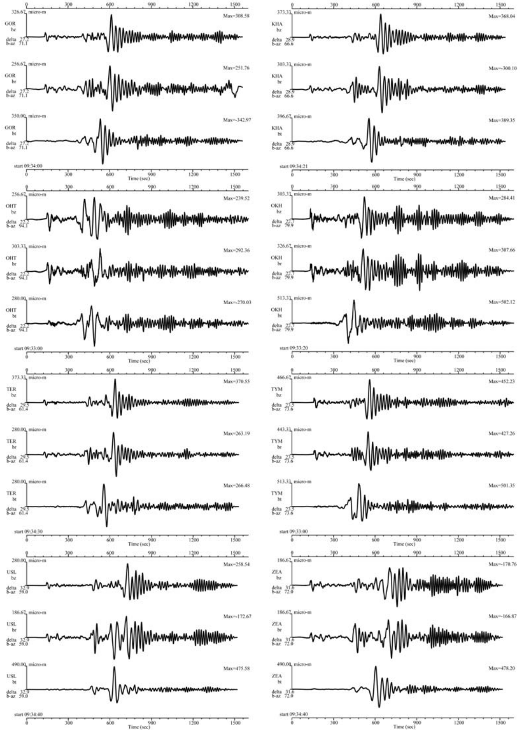
Fig. 5. Seismograms recorded at each station by the Mw 7.2 earthquake occurred at Aleutian Islands on 09h30m, December 19, 2007.
