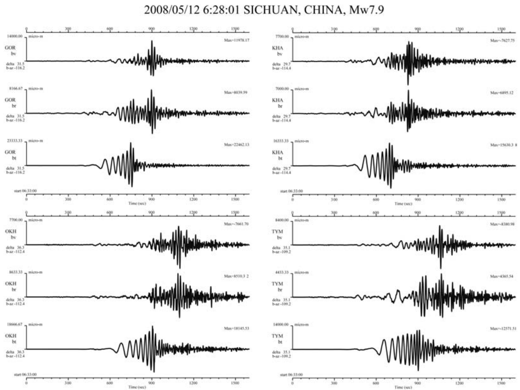
Fig. 7. Seismograms recorded at each station by the Mw 7.9 earthquake occurred in China on 06h28m, May 12, 2008.
