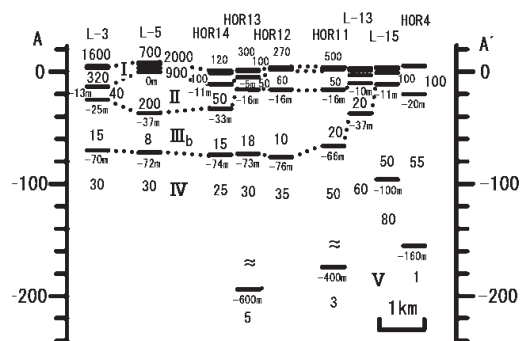
Fig. 3. Two-dimensional resistivity model along the line A-A' in Fig.1. Numbers with "HOR" (ex. HOR4) are survey points in 2005 (Table 1). And numbers with "L" (ex. L-3) are survey points in 2006 (Table 2).
