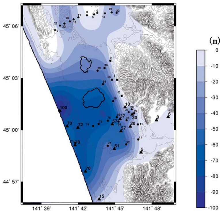
Fig. 7. Contour map of the depth distribution of the layer III. Circles and triangles denote locations of our survey in 2005 and 2006, respectively. Crosses denote survey points by Hokkaido development (1966). Number indicates are the depth of the layer III at each point.
