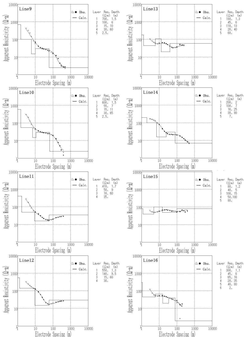
Af. 2-2. Survey results in 2006 and the fit for the Schlumberger sounding curve. And the resistivity structure from the analysis (No.2).
