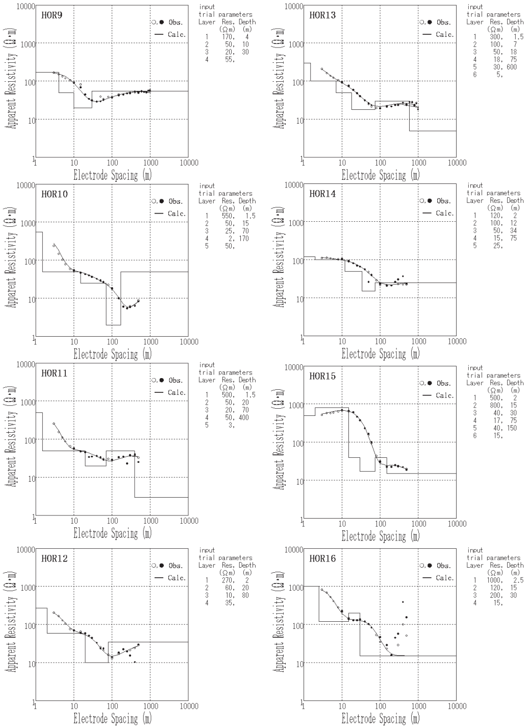
Fig. 1-2. Survey results in 2005 and the fit for the Schlumberger sounding curve. And the resistivity structure from the analysis (No.2).
