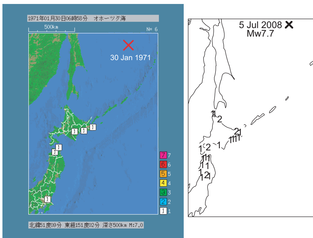
Fig. 5. Seismic intensity distribution for the 1971 and 2008 deep-focus earthquakes in northeastern Okhotsk Sea.
