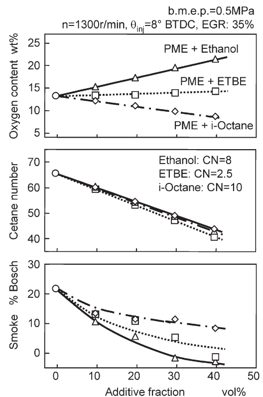
Fig. 12 Influence of oxygen content and cetane number of additive fuels on smoke reduction
