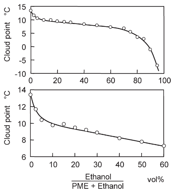
Fig. 1 Cloud point with ethanol-blended PME
