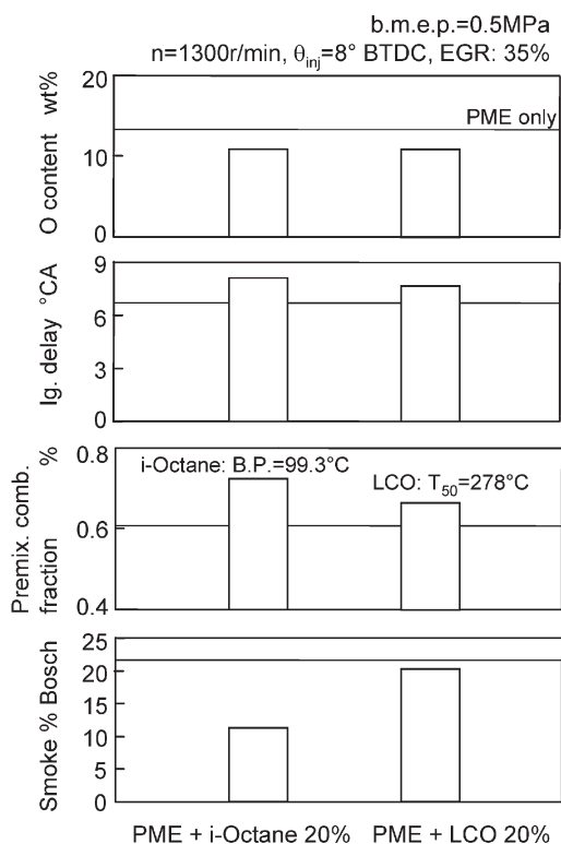
Fig. 13 Influence of volatility of additive fuels on smoke reduction
