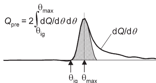
Fig. 15 Estimation of premixed combustion heat release
