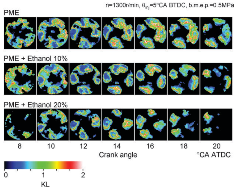
Fig. 11 Distribution of KL factor in ethanol-blended PME combustion flame
