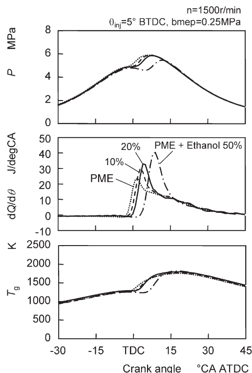
Fig. 3 Influence of ethanol blending on in-cylinder pressure, apparent rate of heat release, and in-cylinder gas mean temperature in PME combustion [5]. ATDC: after top dead centre
