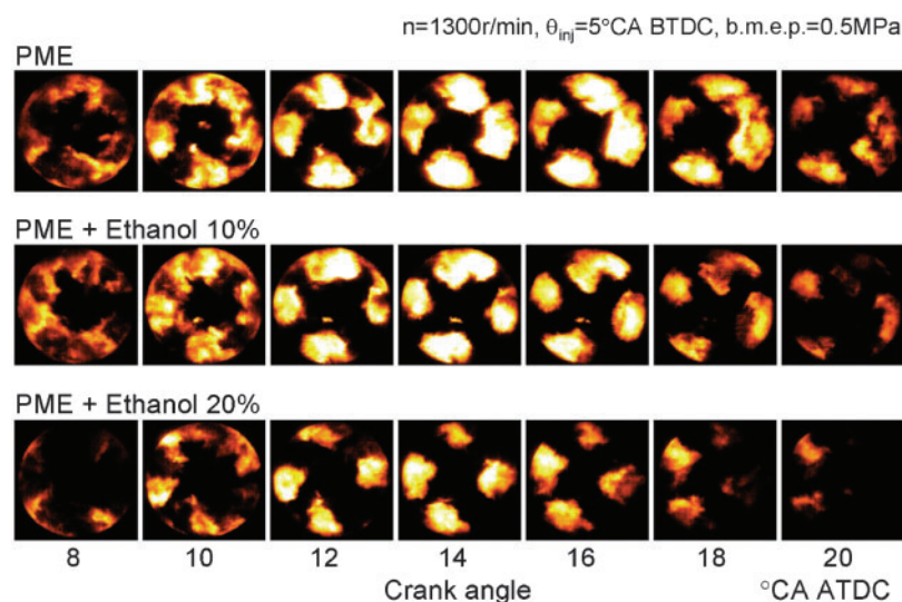
Fig. 8 Flame images of ethanol-blended PME combustion
