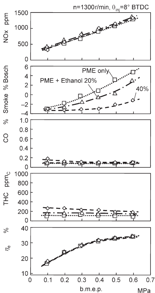
Fig. 2 Influence of ethanol blending on exhaust emissions and thermal efficiency in PME combustion
