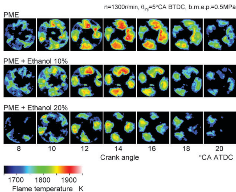
Fig. 10 Flame temperature distribution in ethanol-blended PME combustion
