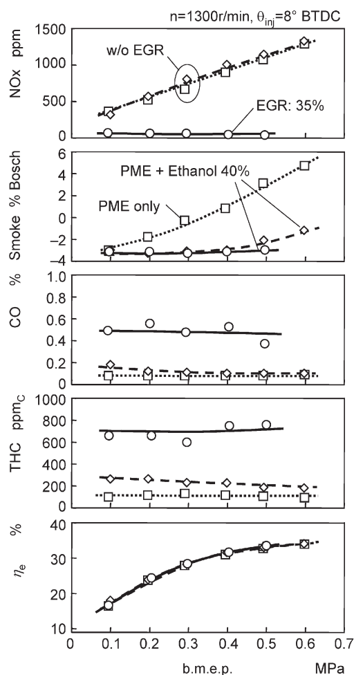
Fig. 5 Influence of ethanol blending and EGR on exhaust emissions and thermal efficiency in PME combustion
