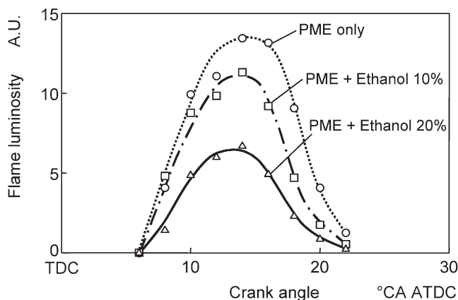
Fig. 9 Influence of ethanol blending on average flame luminosity
