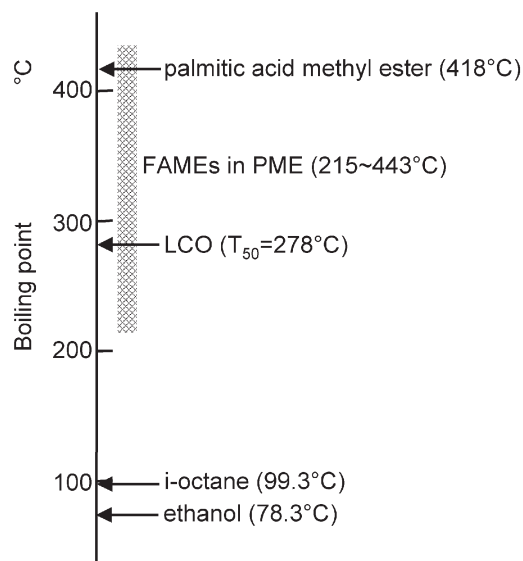
Fig. 14 Volatility of the tested fuels
