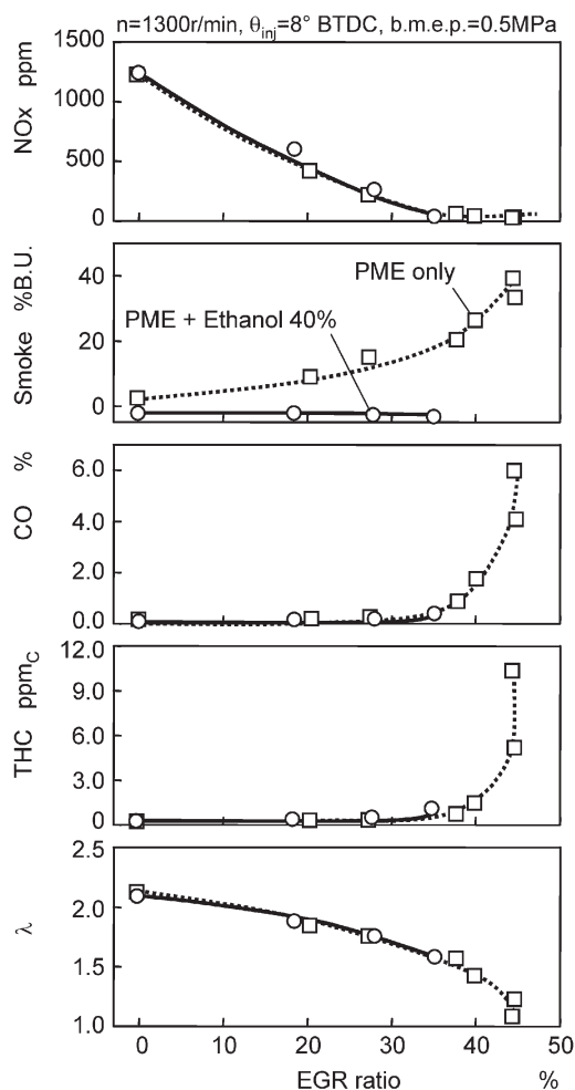
Fig. 6 Influence of EGR on exhaust emissions and thermal efficiency in ethanol-blended PME combustion
