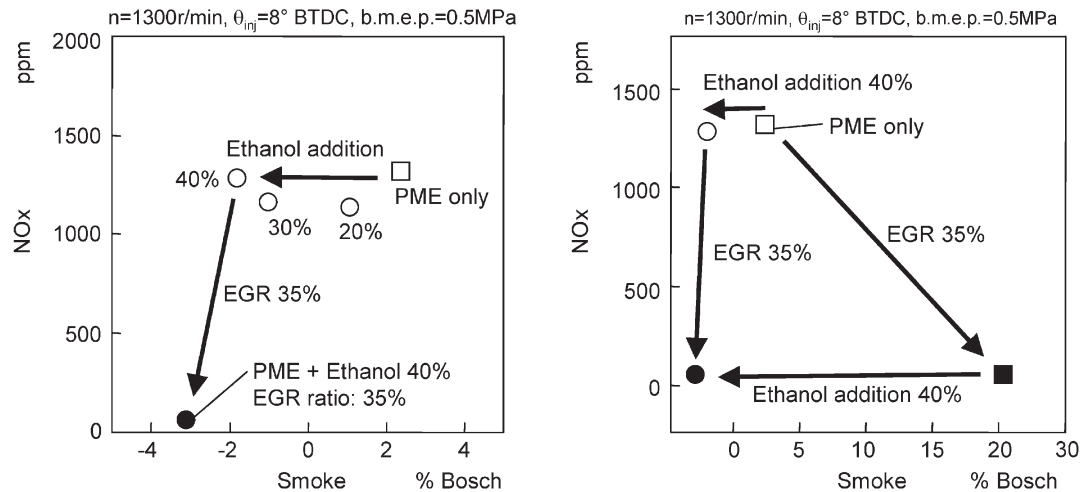
Fig. 7 Influence of ethanol blending and EGR on the NO x and smoke relation
