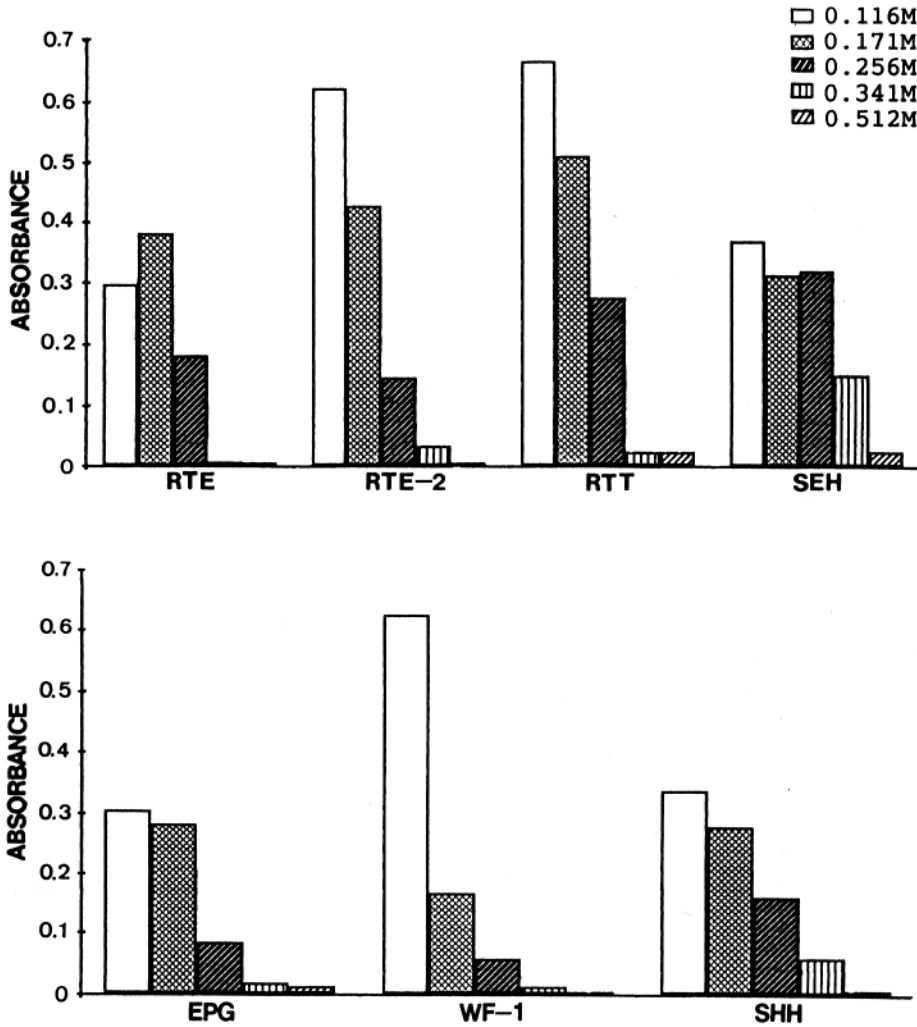
FIGURE 4.—Growth responses of (top) salmonid and (bottom) nonsalmonid cell lines at various NaCl molarities.
