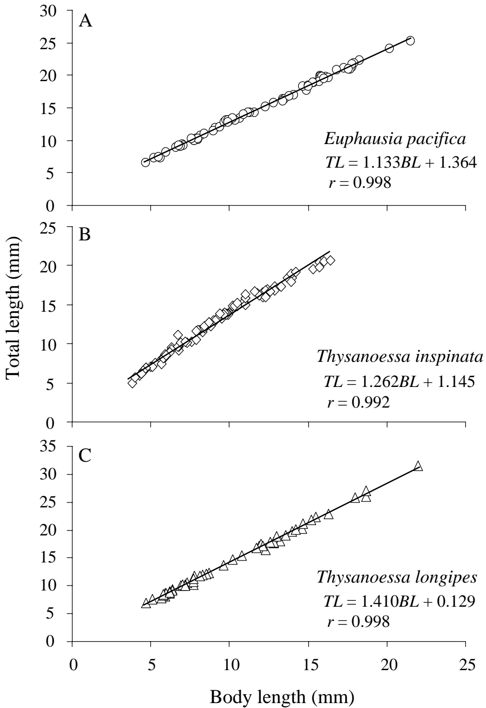
Fig. 3-3. Relationship between total length (TL) and body length (BL) of Euphausia pacifica (A), Thysanoessa inspinata (B) and T. longipes (C) at Site H in the Oyashio region.
