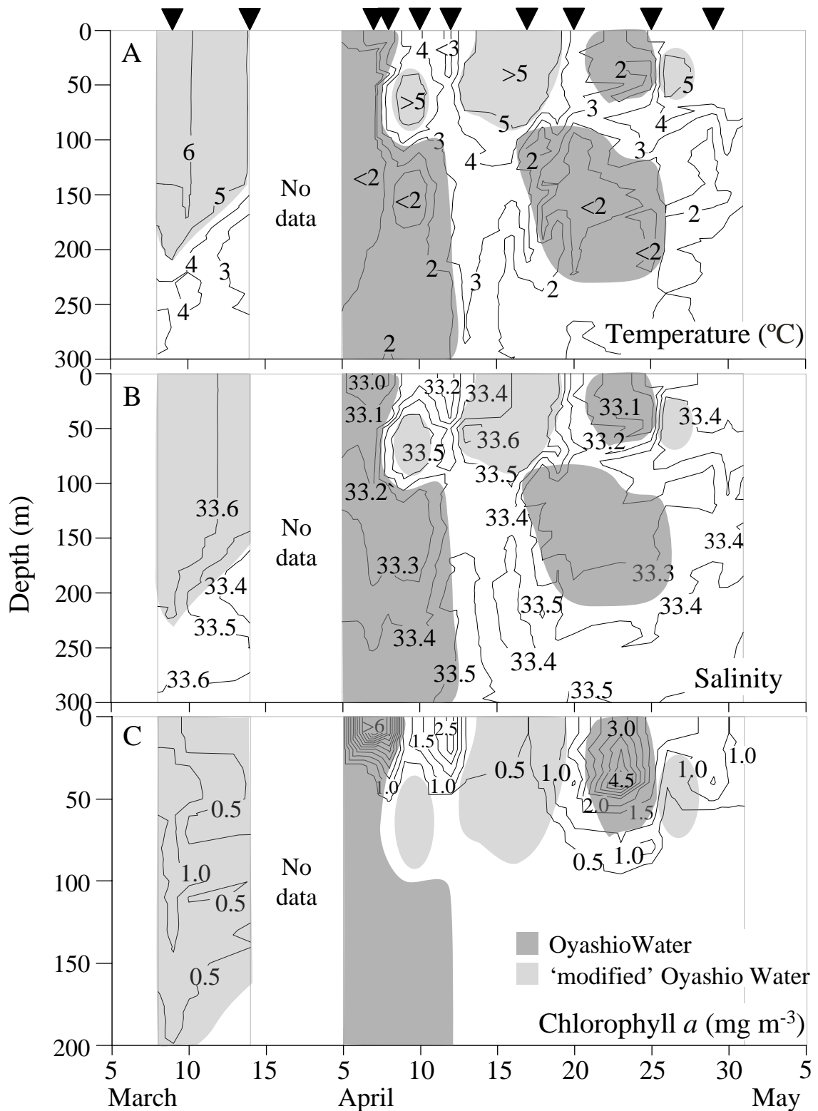
Fig. 4-2. Temporal changes in temperature (A), salinity (B) and chlorophyll a (C) profiles at the station A-5 in the Oyashio region during March to April 2007. Solid triangles in the top abscissa indicate sampling dates. Note that depth scale of (C) is not the same to those of (A) and (B).
