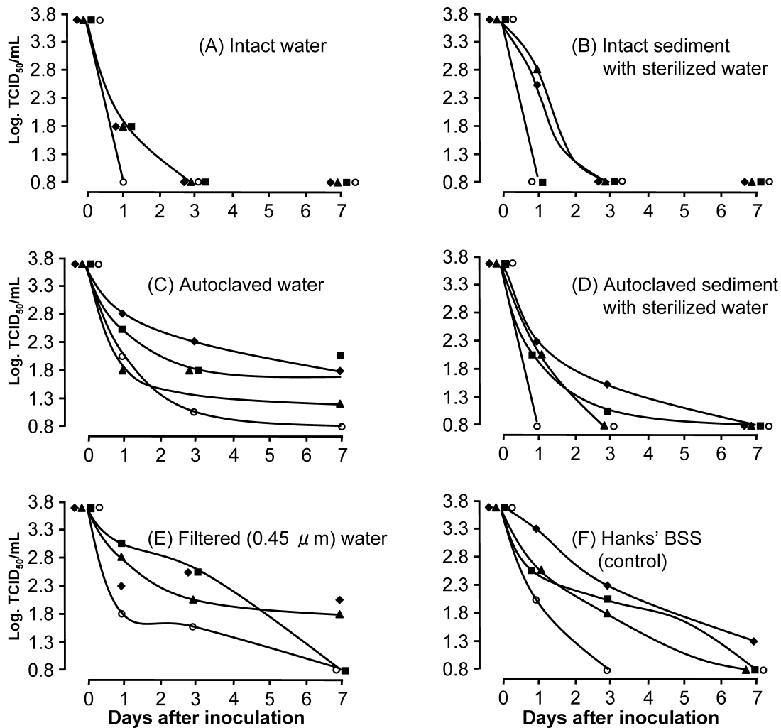
Fig. 2. Changes in infectious titer of KHV in water or sediment collected from Lake Kasumigaura held at 15, 20, 25 or 30°C.
