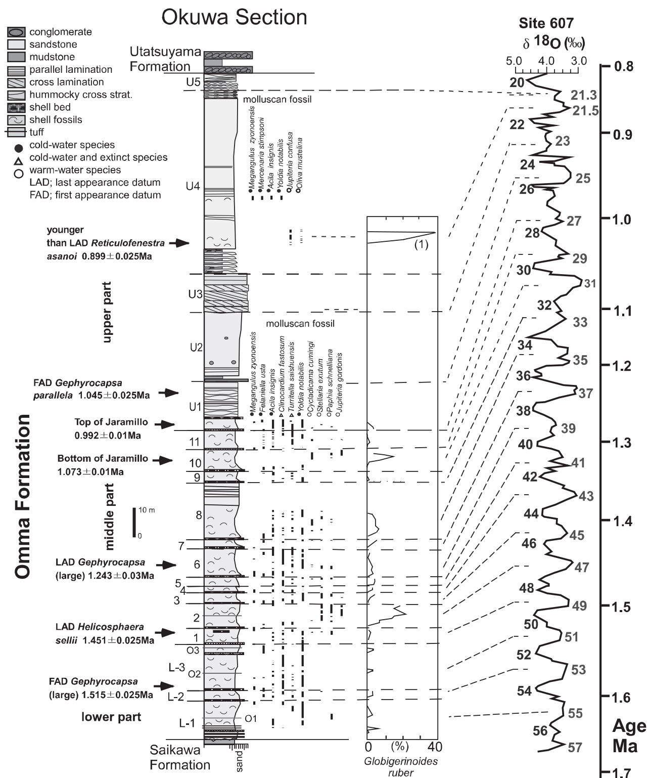
Fig. 2 Columnar section of the Omma Formation at its type section, showing stratigraphic distribution of selected molluscan fossils and the relative abundance of Globigerinoides ruber .
