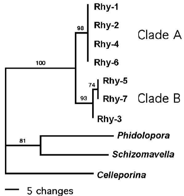
Fig. 1 Single shortest tree from a maximum parsimony analysis of a partial fragment of the 16S mtrRNA gene, including sequences from seven colonies of Rhynchozoon sp. (Rhy-1 to 7) and three outgroup taxa; length = 146 steps, CI (excluding uninformative characters) = 0.8765, RI = 0.8864. Values above branches indicate bootstrap values in percent from 1,000 bootstrap replicates, with replacement.
