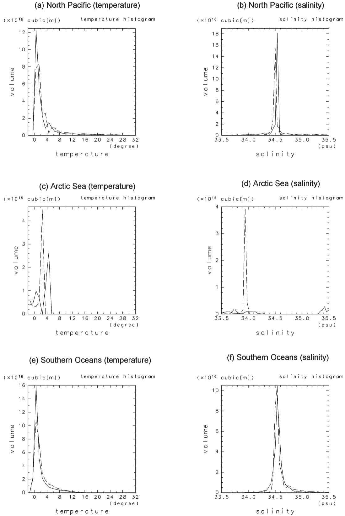
Fig. 3 Histograms of temperature (left) and salinity (right) for North Pacific (top), the Arctic Sea (middle) and the Southern Oceans (bottom), respectively. Solid and dashed lines in each panel depict control and PG runs, respectively.
