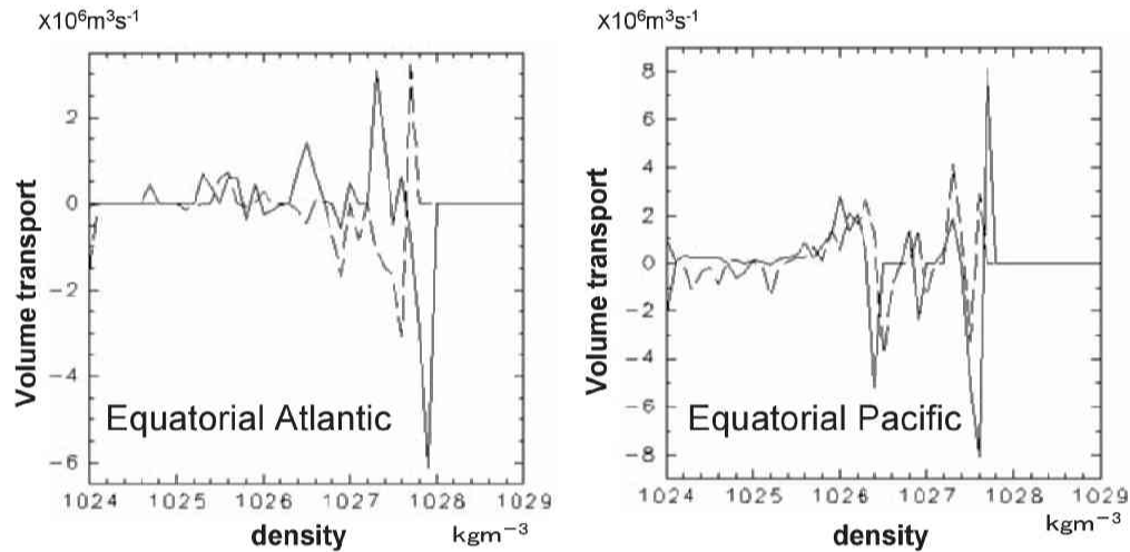
Fig. 5 Density weighted volume transport across the equator. Left: transport across the equator in the Atlantic Ocean (line 5 in Fig. 4); right: transport across the equator in the Pacific Ocean (line 4 in Fig. 4). Solid and dashed lines in each diagram depict the control and PG runs, respectively. Positive and negative values indicate transport northward and southward, respectively.
