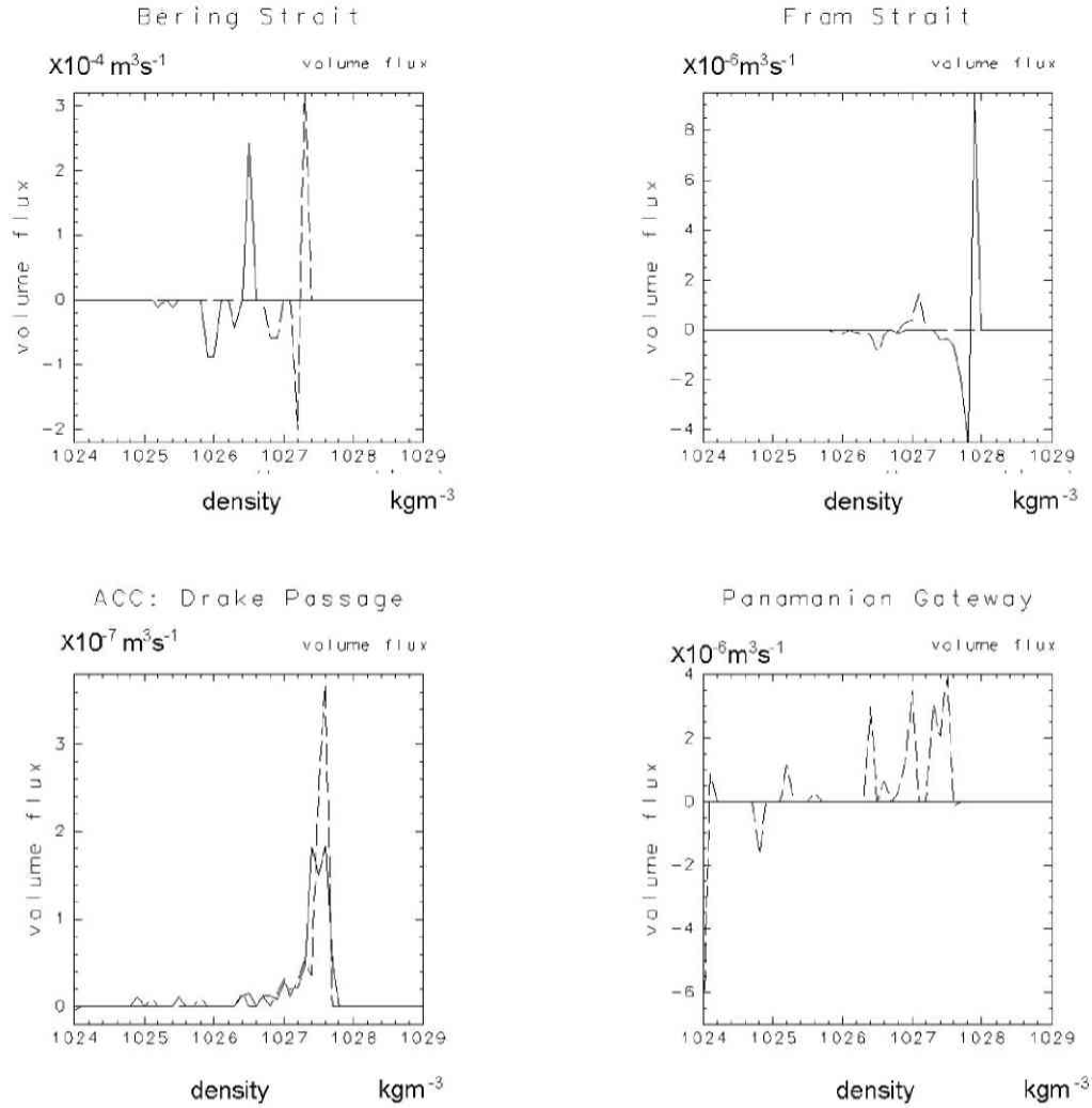
Fig. 6 Density weighted volume transport across the Bering Strait (Fig. 4 section 1), the Fram Strait (Fig. 4 section 2), the Drake Passage (Fig. 4 section 13) and the Panamanian Gateway (Fig. 4 section 14). Solid and dashed lines in each diagram depict the control and PG runs, respectively. Positive value in each figure indicates northward flow except for the Panamanian Gateway. For the Panamanian Gateway, positive value indicates north and eastward flow (flow from the North Pacific to the North Atlantic). Note that the unit of the volume flux is different in each diagram.
