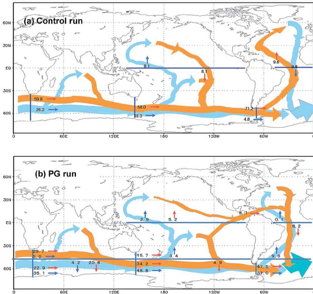
Fig. 7 Schematics of the oceanic conveyor belt in the control run (a), and the PG run (b). In both diagrams, blue and orange belts depict deep (cold) and shallow (warm) water pathways, respectively. Numbers accompanied by small arrows depict the volume transport in the upper (red arrow) or the lower (blue arrow) layer. The unit of the numbers is Sverdrup ( 10^6 \text{ m}^3 \text{ s}^{-1} ).
