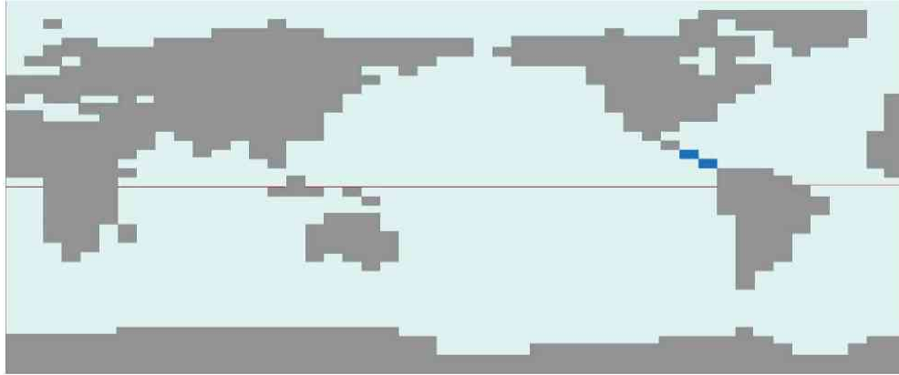
Fig. 1 Model topography [13]. Realistic topography is employed in the control run. After the opening of the Panamanian Gateway, the blue grid boxes are set to be ocean. The depth of the gateway is set to be approximately 2.5 km.
