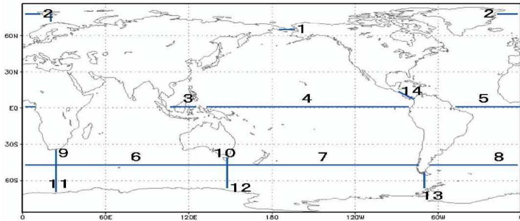
Fig. 4 Inter-ocean sections where density weighted volume transport is calculated. 1. Bering Strait, 2. Fram Strait, 3. Indonesian Strait, 4. Equatorial Pacific, 5. Equatorial Atlantic, 6. Southern Indian Ocean, 7. Southern Pacific, 8. Southern Atlantic, 9. South of Africa, 10. South of Australia, 11. ACC south of Africa, 12. ACC south of Australia, 13. Drake Passage, 14. Panamanian Gateway.
