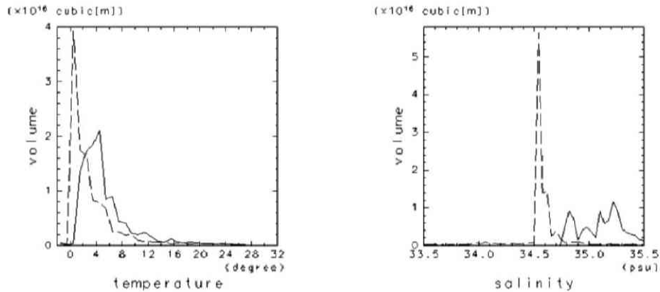
Fig. 2 Histograms of temperature (left) and salinity (right) in the North Atlantic. In both diagrams, solid and dashed lines depict control run with the closed Panamanian Gateway and another run with the opened gateway (PG run), respectively.
