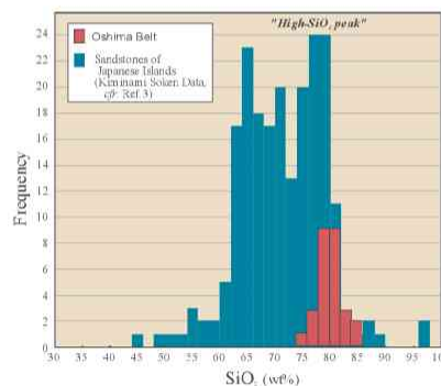
Fig. 6 SiO 2 frequency of Oshima sandstone
