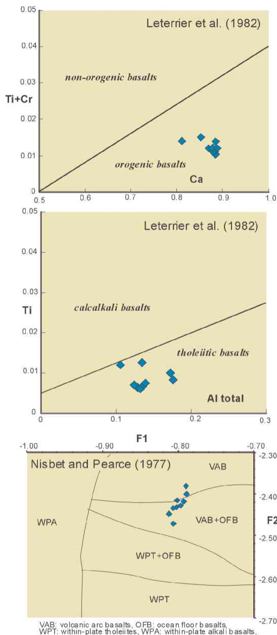
Fig. 13 Composition of detrital clinopyroxene of the sandstone of Karakawa Unit
