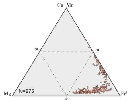
Fig. 8 Composition of detrital garnets of Oshima sandstone
