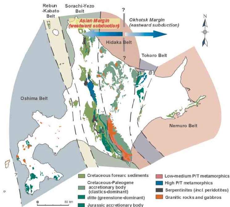
Fig. 1 Pre-Eocene geologic division of Hokkaido
