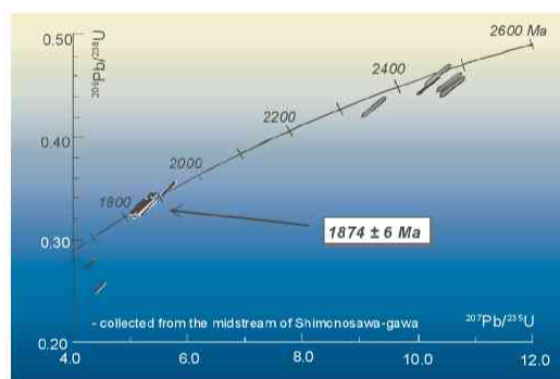
Fig. 9 SHRIMP age of the detrital zircon of Oshima sandstone
