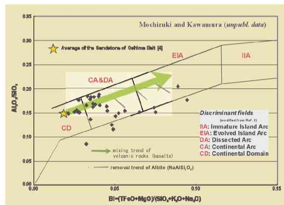
Fig. 12 Chemical composition of the Lower Yezo sandstone and mixing simulation
