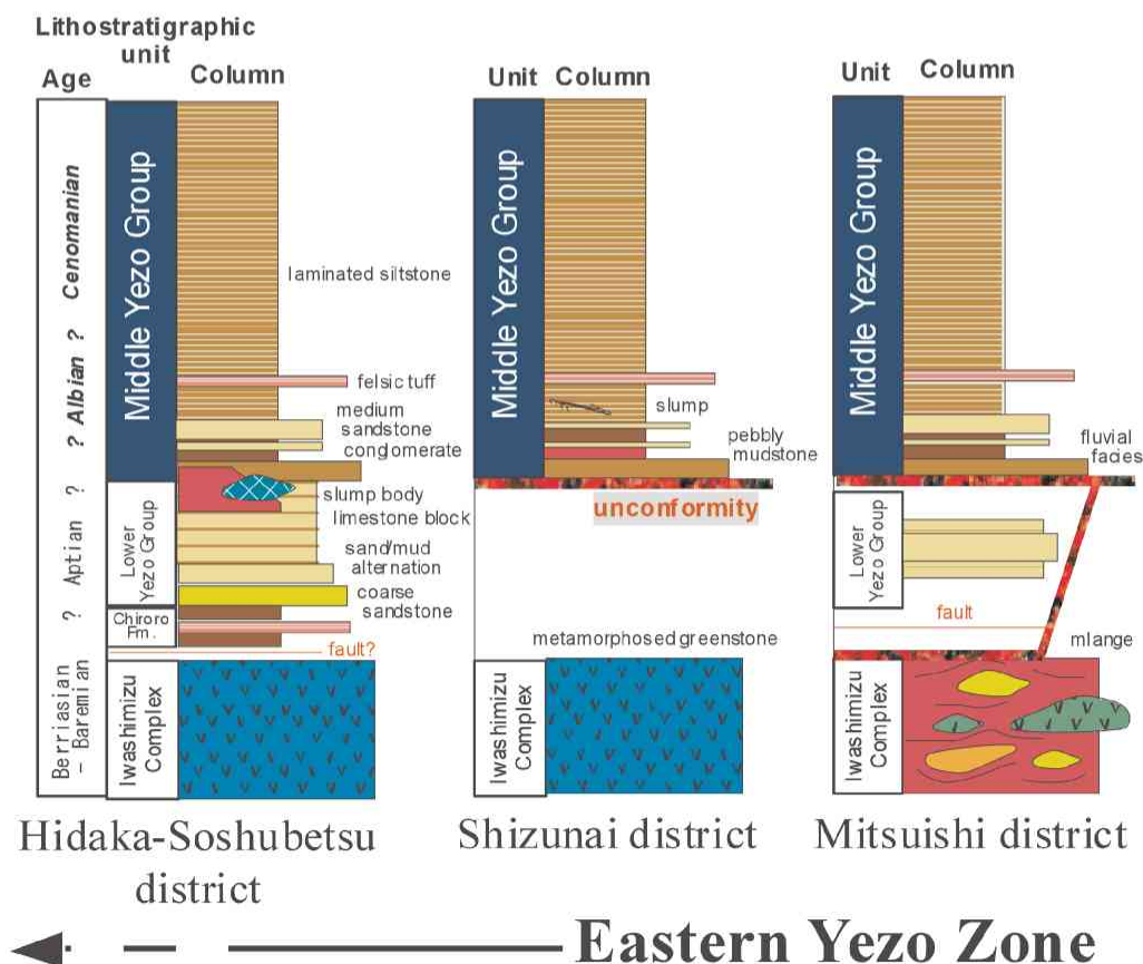
Fig. 17 Stratigraphic scheme of Eastern Yezo Zone
