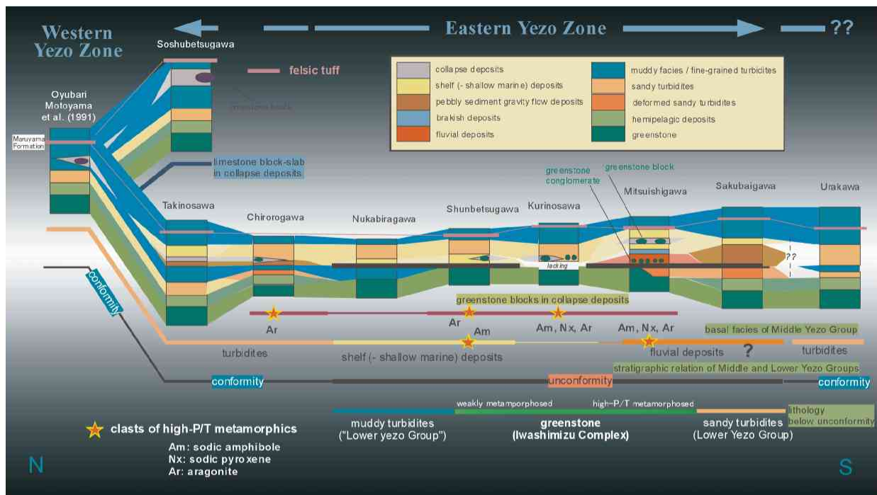
Fig. 18 Lithostratigraphic summary in the Eastern Yezo Zone
