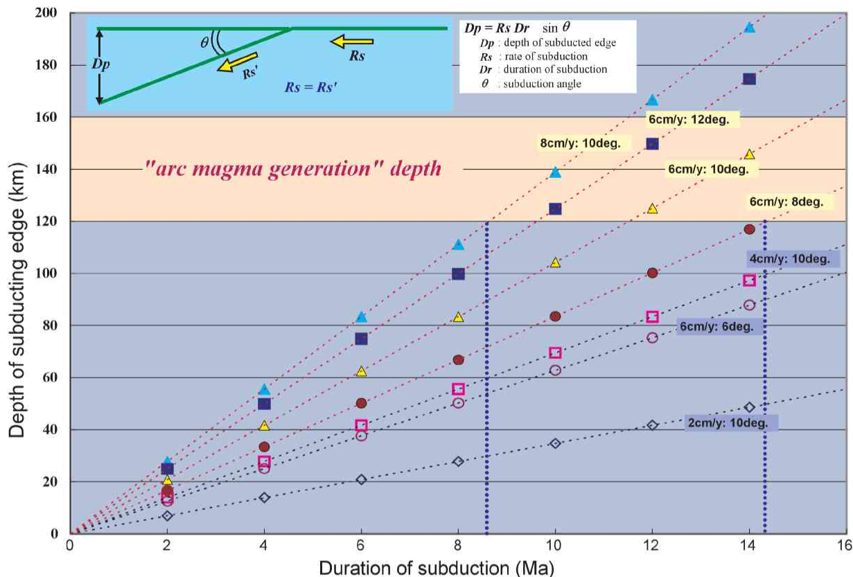
Fig. 14 Depth of the subducted plate
