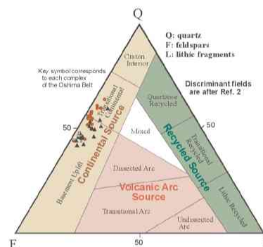
Fig. 5 QFL mode diagram of Oshima sandstone
