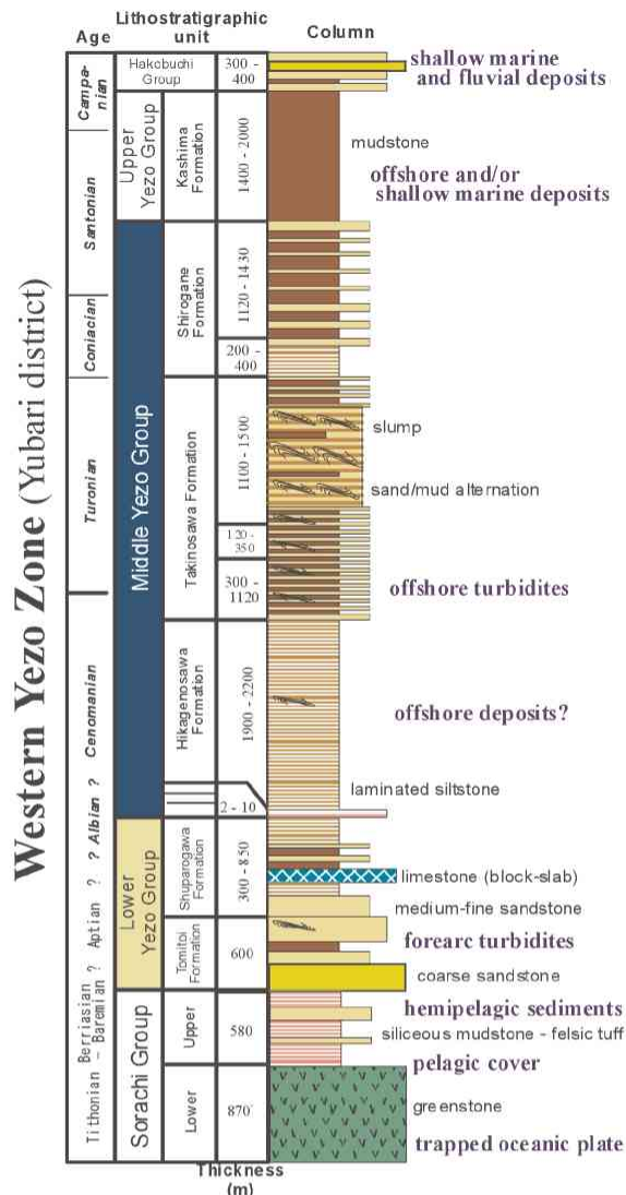
Fig. 11 General stratigraphic column of Yezo Supergroup. Modified after Ref. 6.
