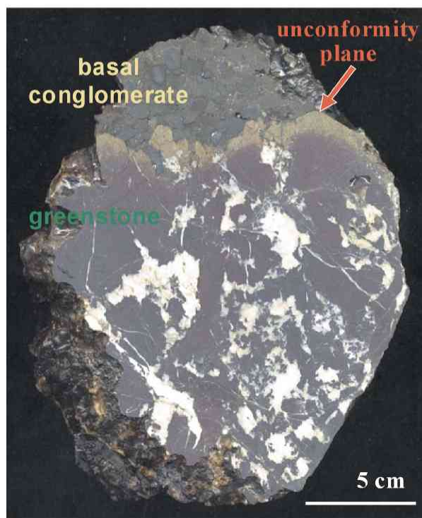
Fig. 15 Specimen of Middle Yezo Unconformity
