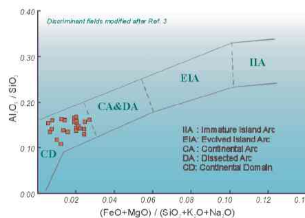
Fig. 7 Oshima sandstone in Kiminami Diagram
