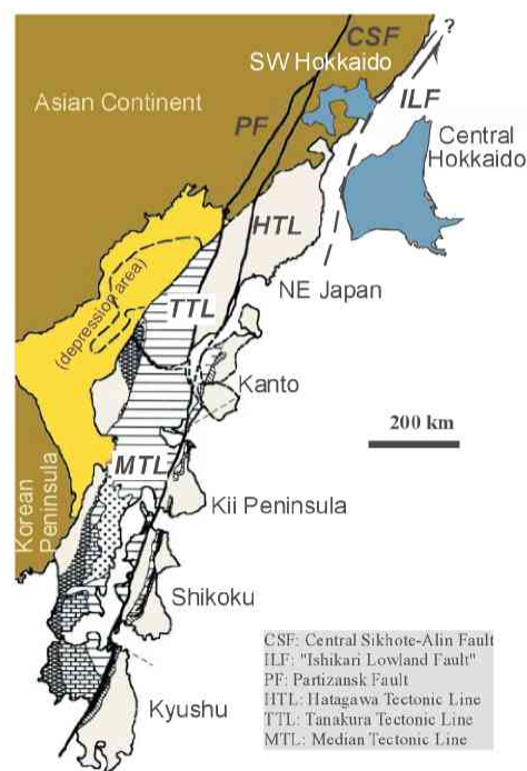
Fig. 10 Pre-Neogene reconstruction of Japanese Islands. Modified after Ref.5.
