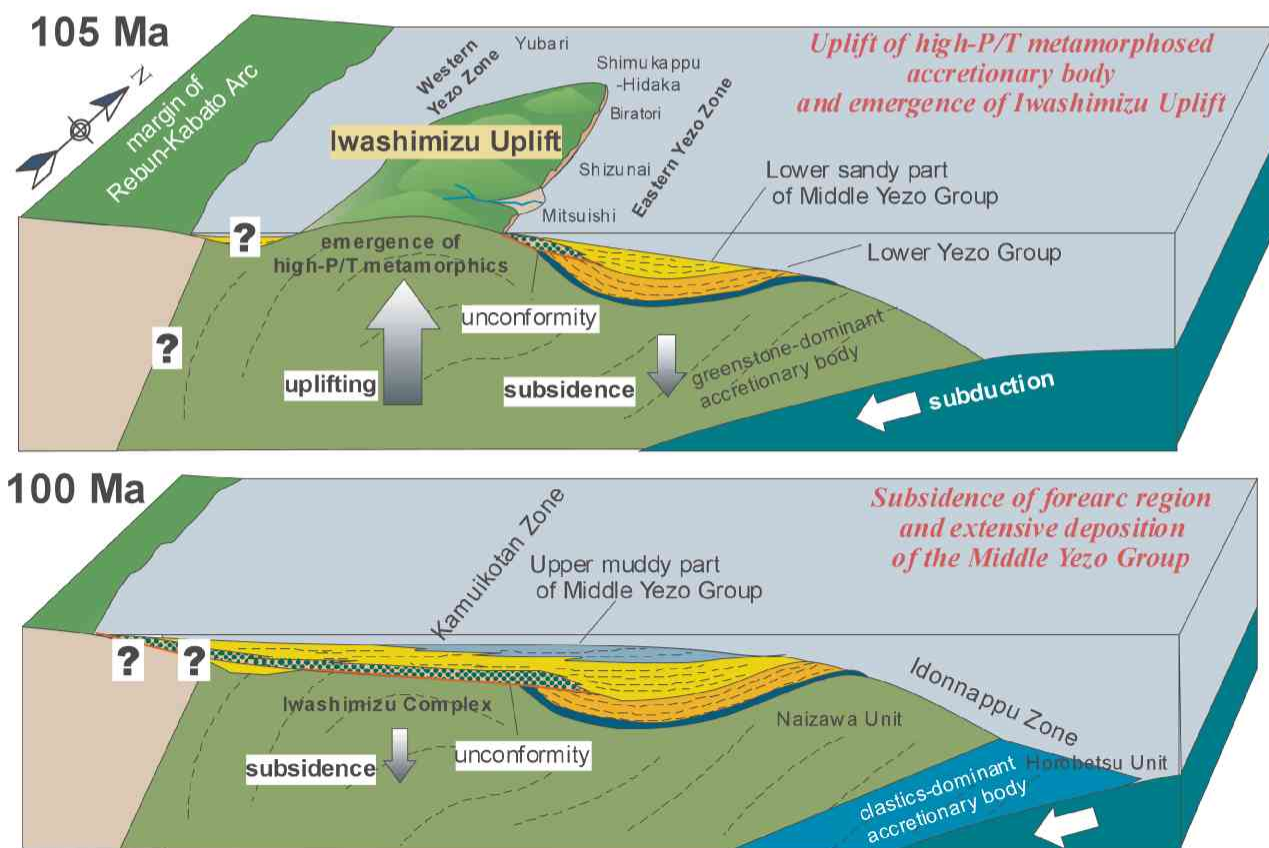
Fig. 19 Model of Middle Yezo Unconformity
