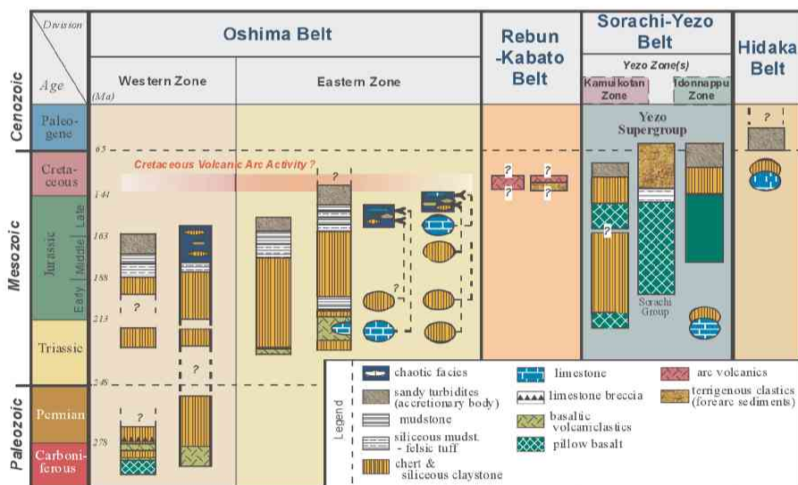
Fig. 2 Tectonostratigraphy of pre-Eocene Hokkaido
