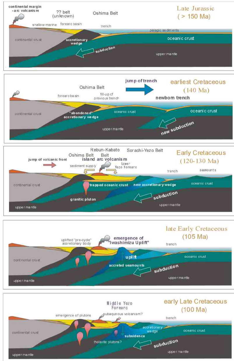
Fig. 3 Plate-tectonic scheme of Jurassic - Cretaceous Hokkaido
