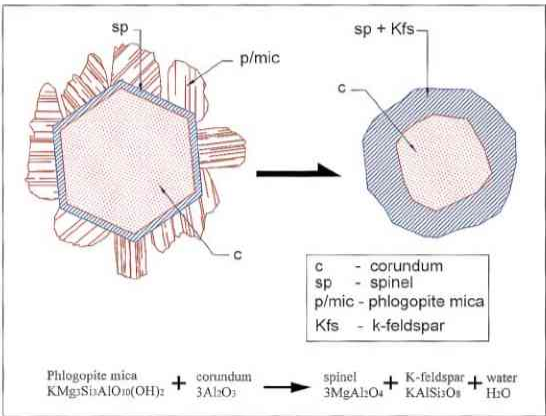
Fig. 5 Schematic illustration of the non-uniform enlargement of spinel rim due to the reaction of corundum and phlogopite (after Ref. 9).
