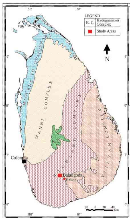
Fig. 1 Geological map illustrating the distribution of crustal units of Sri Lanka (modified after Ref. 2).
