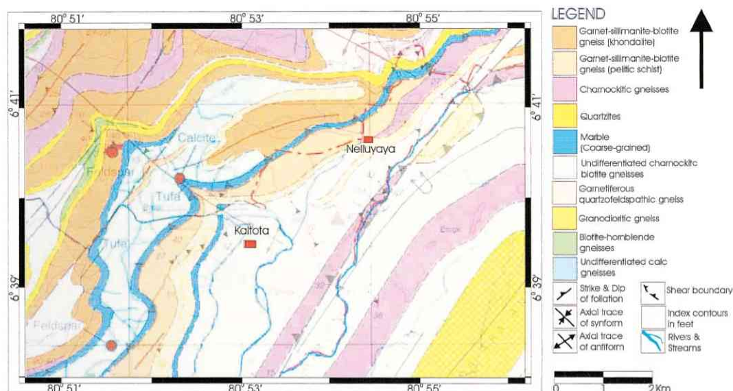
Fig. 2 Geological map of the Kaltota area (Source - GSMB 1 : 100,000 map of Nuwara Eliya- Haputale, after Ref. 6).
