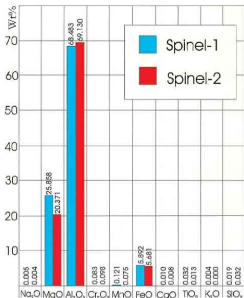
Fig. 6 Comparison of the spinel compositions of the specimens, representing the stages before (Spinel-1) and after (Spinel-2) the reaction.
