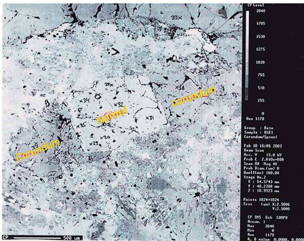
Fig. 7 A small protruded part of spinel rim with microscopic remains of corundum, subjected to backscattered imaging.
