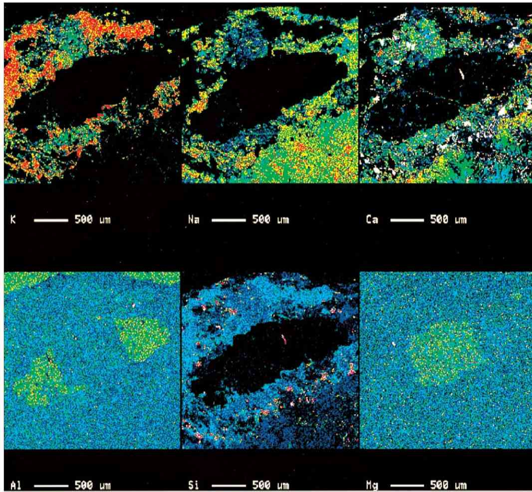
Fig. 8 Element distribution map illustrating the formation of spinel as a byproduct of the reaction between phlogopite mica and corundum. Red and yellow areas within the K map, indicate K rich areas, probably containing phlogopite.
