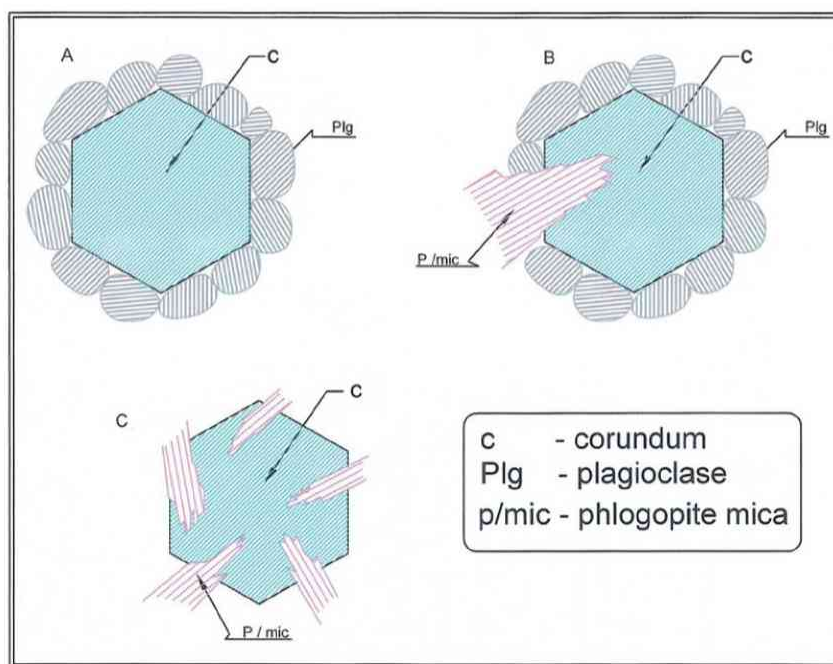
Fig. 11 Schematic illustration of the plagioclase shielding effect over corundum (after Ref. 10).
