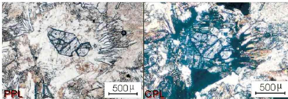
Fig. 9 Photomicrographs illustrating a corundum crystal surrounded by re-crystallized plagioclase grains.
