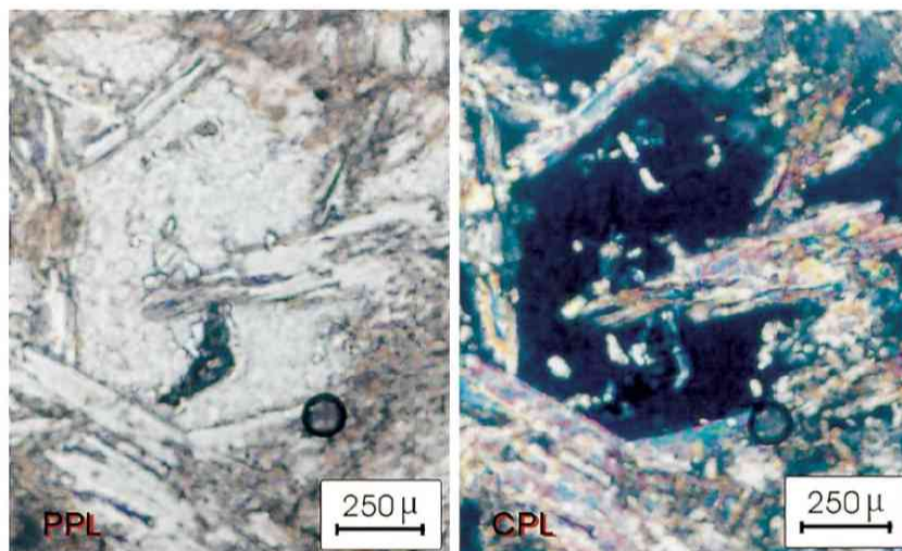
Fig. 10 Photomicrographs illustrating corundum partially surrounded by re-crystallized plagioclase grains. The portion of corundum devoid of plagioclase rim is subjected to the reaction process of phlogopite mica formation.
