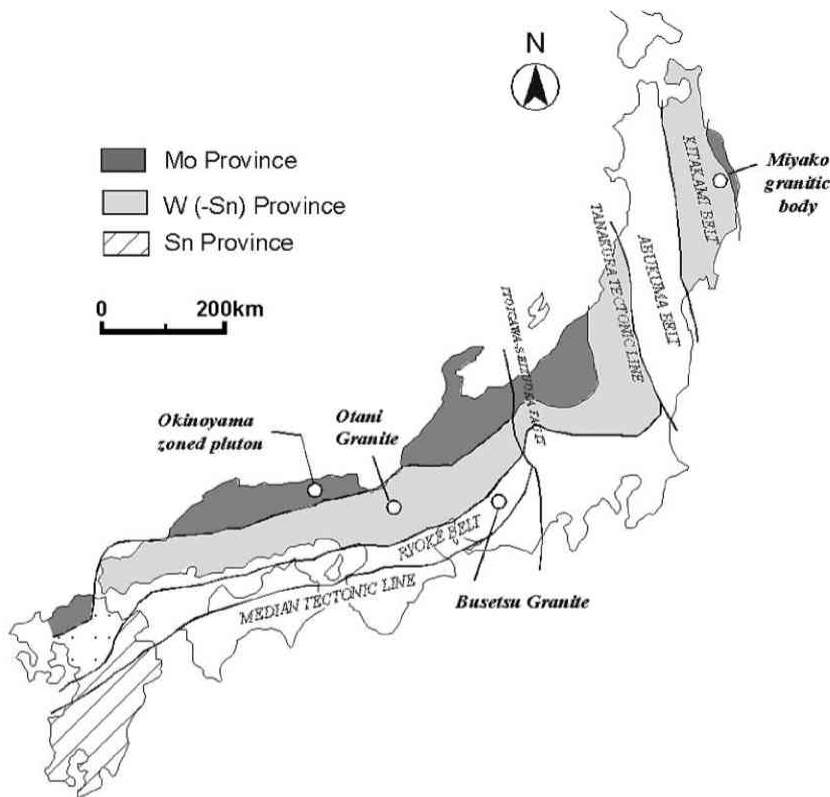
Fig. 1 Molybdenum and tungsten-tin metallogenic zoning of the Japanese islands (after Ishihara [6]).
