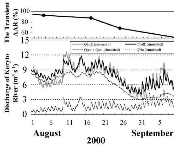
Fig. 5 Measured and simulated discharge of Koryto River and the variation in the transient accumulation area ratio (AAR) in the summer of 2000. Thick grey line and thick black line indicate measured and simulated bulk meltwater discharge. Thin line and dotted line indicate the component of meltwater from the snow-covered area plus stored water within the glacier, and the component of meltwater from bare ice area.
