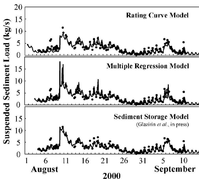
Fig. 7 Simulated suspended sediment load of Koryto River using the rating curve model, the multiple regression model and the sediment storage model.
