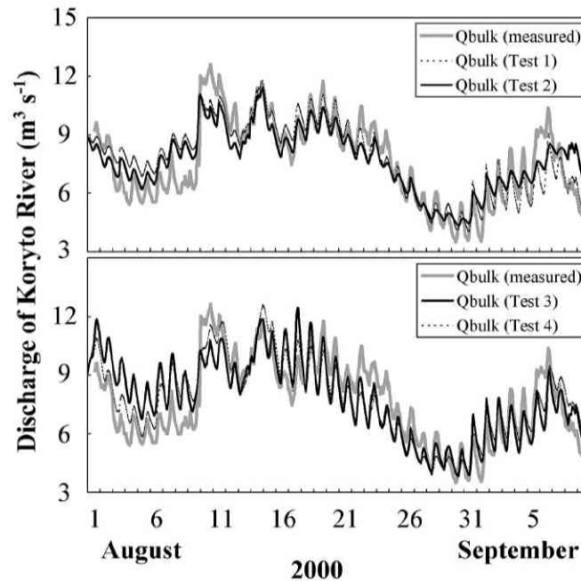
Fig. 6 Results of runoff model simulation with different assumptions on spatial changes in the transient snowline. Test 1: assuming the measured snowline retreat, Test 2: assuming fixed snowline at the height on August 1 (tuned coefficients), Test 3: assuming fixed snowline at the height on September 1 (tuned coefficients), Test 4: assuming fixed snowline at the height on September 1 (the same coefficients as those of Test 1).
