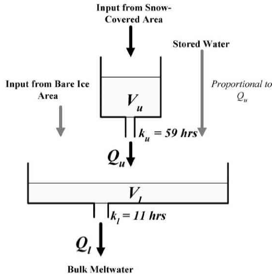
Fig. 4 Schematic representation of the linear reservoir model adopted for Koryto Glacier basin.
