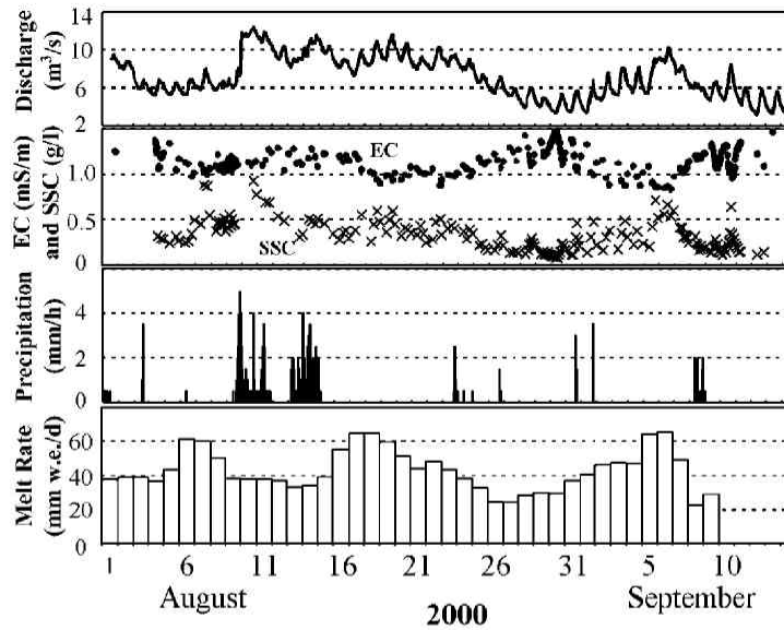
Fig. 2 Variations in discharge, electric conductivity (EC) and suspended sediment concentration (SSC) of Koryto River, precipitation at the site HS and the area-weighted mean melting rate of Koryto and Kudelyko Glaciers in the summer of 2000.
