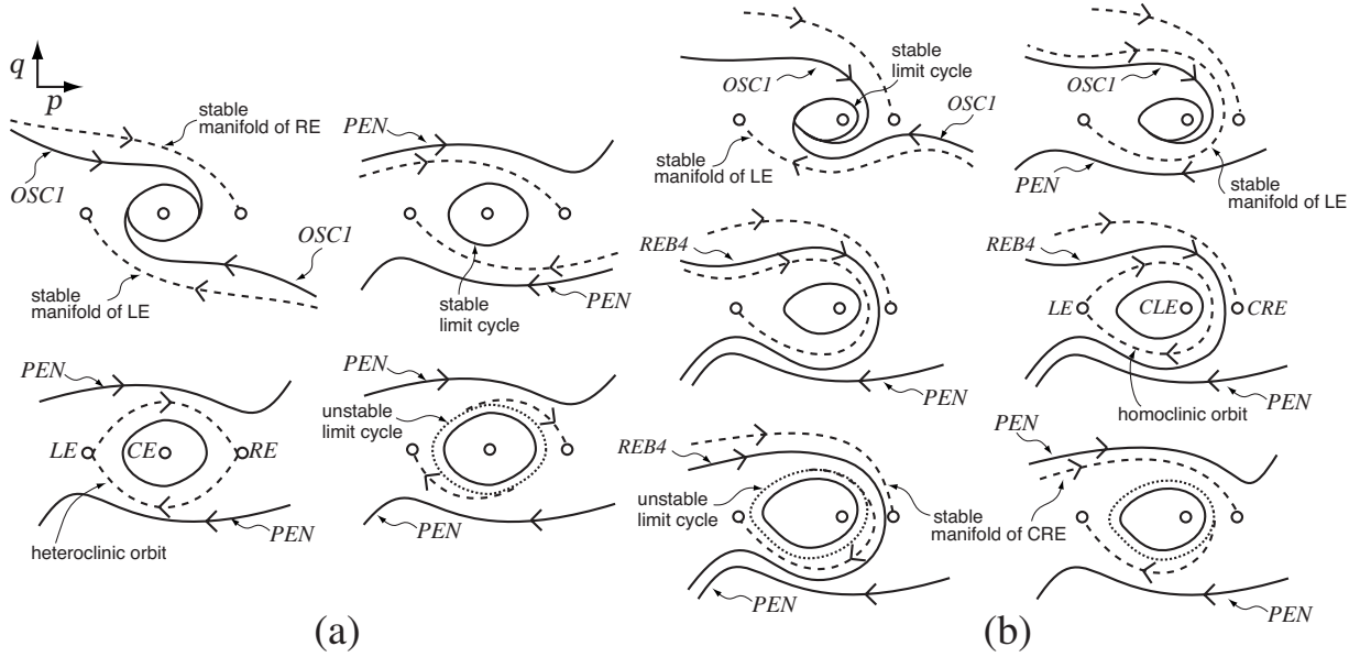
FIG. 11. The schematic orbit flows explain how the change of type of global bifurcation causes the RECT1 and unOSC1 behaviors between bidirectional behaviors for positive \epsilon region. (a) For the symmetric case, bidirectional oscillatory pinning (biOSC) behavior changes into biPEN behavior via a double heteroclinic bifurcation from left-top to right-bottom pictures by decreasing \epsilon . (b) The heterogeneous media are changed from symmetric to asymmetric; double heteroclinic loop is transformed into homoclinic one. The unidirectional oscillatory pinning behavior (unOSC1) and the rectification to the left (RECT1) behaviors occur between bidirectional behaviors as \epsilon is decreased from left-top to right-bottom pictures. The lower-right stable manifold of LE plays a role of scatterers at transitions from biOSC to unOSC1 and from unOSC1 to RECT1, respectively. As \epsilon is still decreased, the upper-left stable manifold of CRE becomes the scatterer at transition between RECT1 and biPEN [see Fig. 6(a)]. The solid (broken) lines indicate the orbit flows from E_2^\pm (p = \mp \infty) (stable manifold of critical points). The solid (dotted) circles show the stable (unstable) limit cycles and the white circle indicates the unstable critical points.
