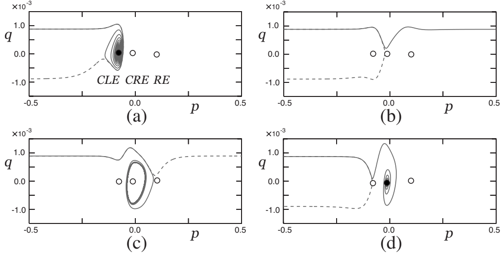
FIG. 4. Orbit flows in (p, q) space for d = -0.10 are depicted in (a) for transition from STA1 to REB1 around \epsilon \approx 0.124 near point F in Fig. 2(b), (b) for transition from REB1 to PEN around \epsilon \approx 0.047 near point G , (c) for transition from PEN to OSC2 around \epsilon \approx -0.073 near point H , and (d) for transition from STA2 to REB2 around \epsilon \approx -0.182 near point I . The solid and open circles indicate the stable and unstable stationary states, respectively.
