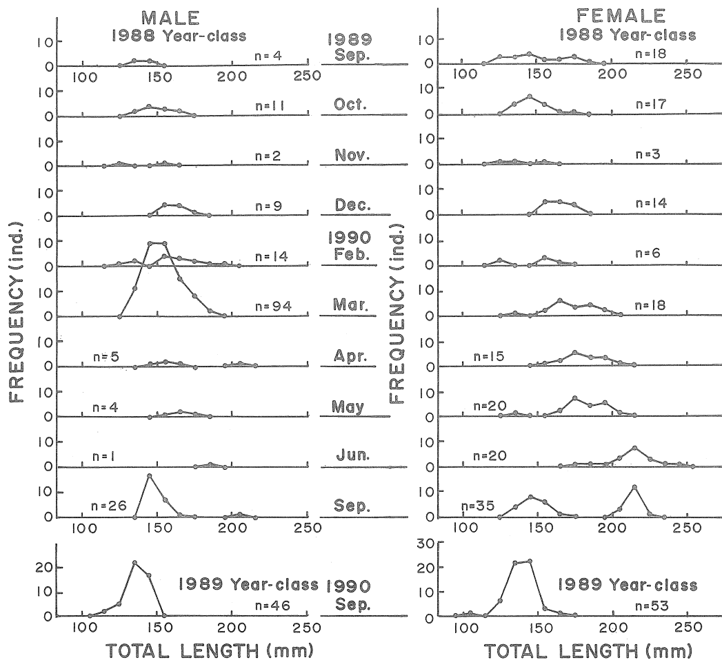
Fig. 5. Length frequency distributions for the 1988 year-class of brown sole collected from September 1989 to September 1990. Data for the 1989 year-class collected in September 1990 are also shown. n: number of fish examined.
