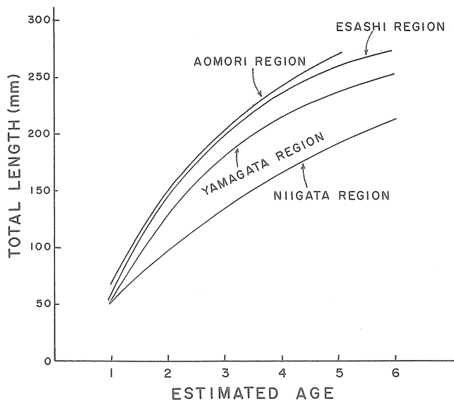
Fig. 7. Comparison of female brown sole growth curve for this study area with those for Niigata region given by Wada, 2) for Esashi region by Nishiuchi, 3) and for Yamagata region by Sando and Hida. 10)
