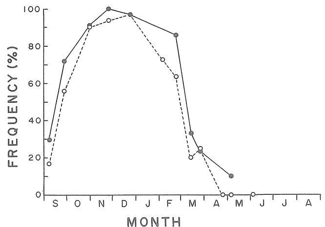
Fig. 3. Percentage occurrences of otolith with translucent edge in male (solid circles) and female (open circles) brown sole.
