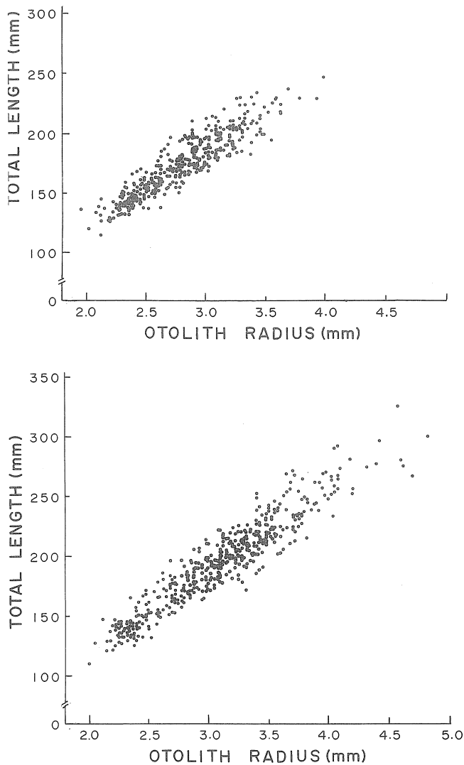
Fig. 4. Relationships between otolith radius and total length for male (upper) and female (lower) brown sole.
