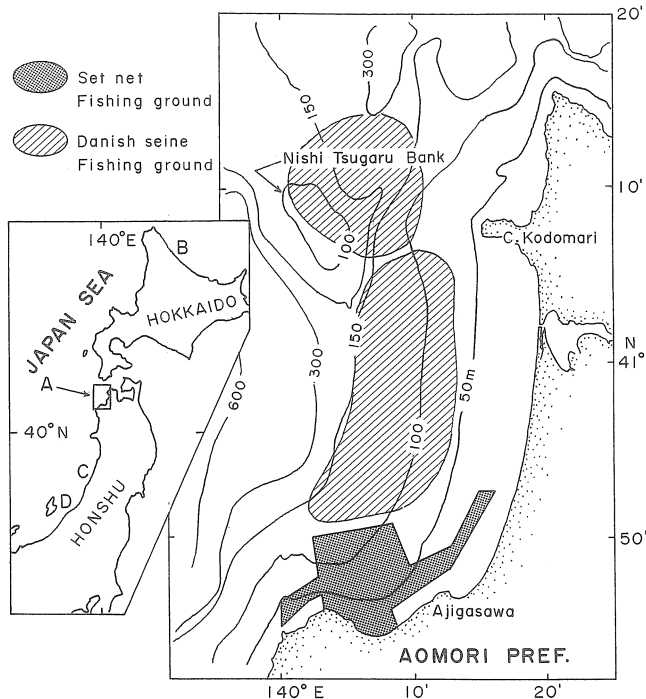
Fig. 1. Map showing sampling area (shaded and striped parts) and contours of depth (m) in the coastal waters of western Aomori Prefecture.
