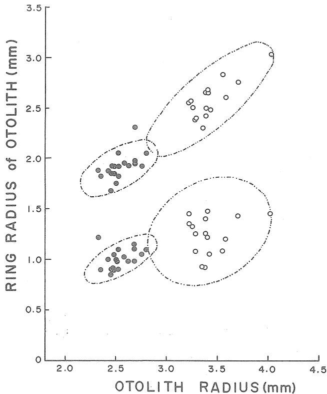
Fig. 6. Rejection ellipses for relationships between otolith radius and ring radius ( r_1 \sim r_2 ) for two-year-old female brown sole collected in September 1990.
