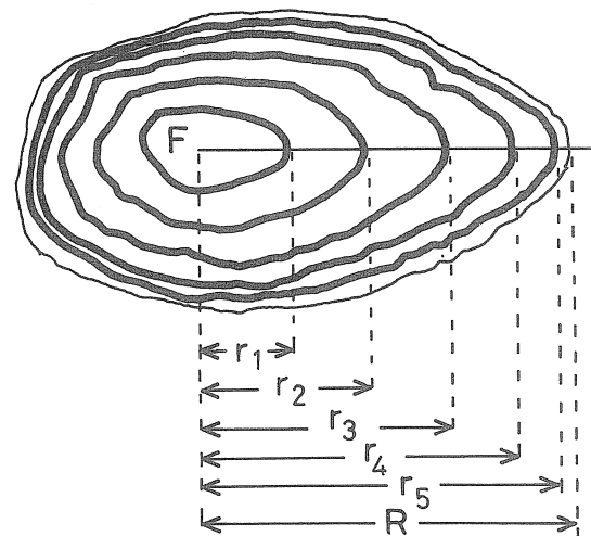
Fig. 2. Ocular side otolith of brown sole with five annuli (female, 280 mm in total length).
