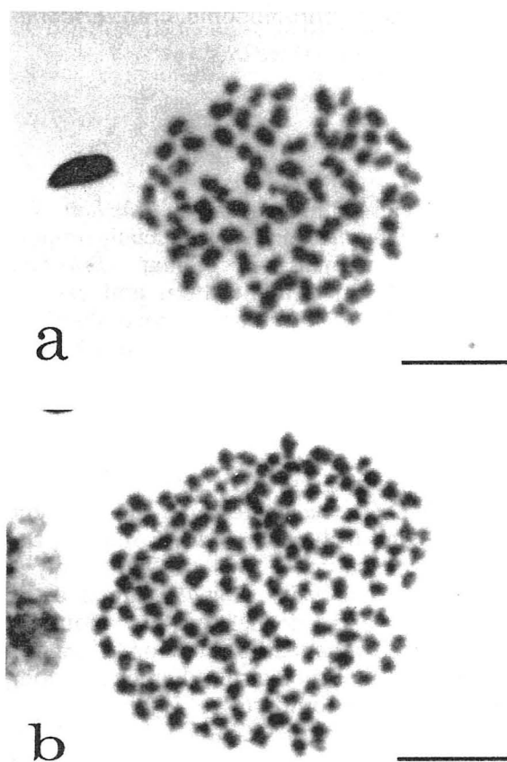
Fig. 1 Metaphase chromosomes obtained from testes of Eriocheir japonica . (a) Meiotic chromosomes; (b) mitotic chromosomes. Bars = 10 µm.
