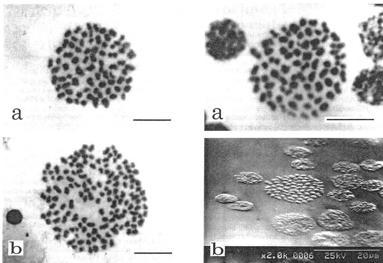
Fig. 2 Metaphase chromosomes obtained from testes of Eriocheir sinensis . (a) Meiotic chromosomes; (b) mitotic chromosomes. Bars = 10 \mu m.
