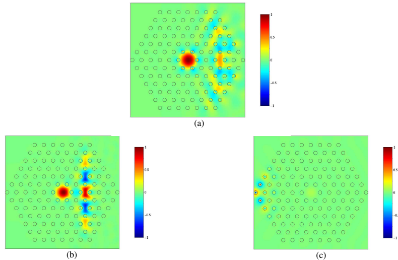
Fig. 4. x -component of electric field distributions of horizontally polarized modes at the bend radius corresponding to the first appearance of the complete mode coupling (in Fig. 3) for the (a) blue-edge, (b) mid-gap, and (c) red-edge wavelengths, respectively. The rod modes consist of LP_{12} mode for blue-edge and mid-gap, and LP_{02} mode for red-edge wavelength, respectively.
