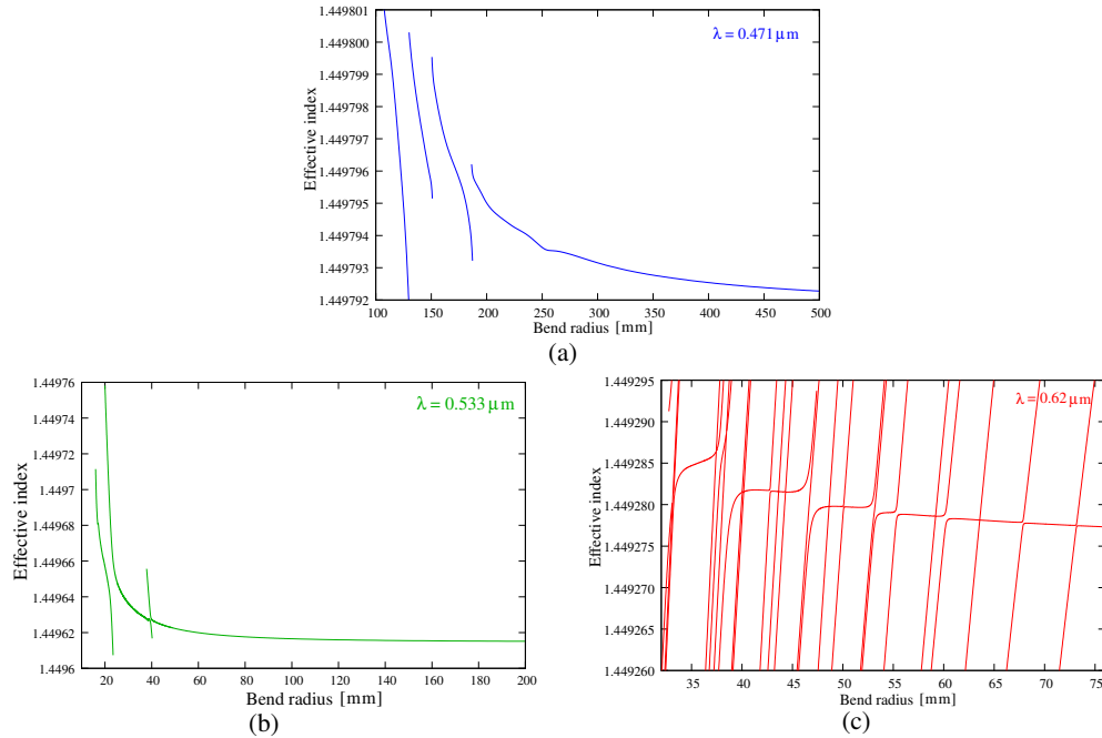
Fig. 3. Bend-radius dependence of the effective refractive indices of the modes for the (a) blue-edge, (b) mid-gap, and (c) red-edge wavelengths, respectively.
