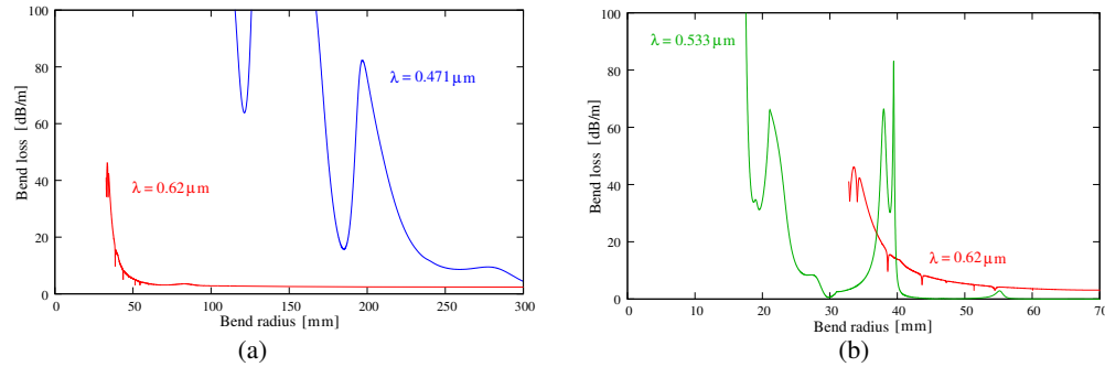
Fig. 8. Bend losses as a function of bend radius for the fiber with 5 cladding rings for (a) blue-edge and red-edge wavelengths, and for (b) mid-gap and red-edge wavelengths, respectively.
