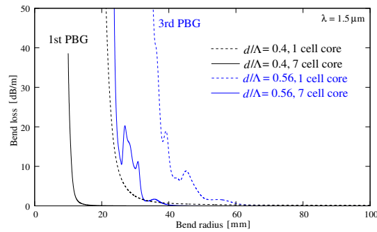
Fig. 13. Bend losses as a function of bend radius for the fibers with d/\Lambda = 0.4 , \Lambda = 6.75 \mu\text{m} , 7 cell core and 5 cladding rings (solid black curve), and with d/\Lambda = 0.56 , \Lambda = 13.5 \mu\text{m} , 1 cell core and 6 cladding rings (dashed blue curve) at \lambda = 1.5 \mu\text{m} (mid-gap wavelength of the fibers). The core radius relative to wavelength is almost identical for the fibers. As a reference, bend losses for the fibers with d/\Lambda = 0.4 , \Lambda = 6.75 \mu\text{m} , 1 cell core and 6 cladding rings (dashed black curve), and with d/\Lambda = 0.56 , \Lambda = 13.5 \mu\text{m} , 7 cell core and 5 cladding rings (solid blue curve) are also depicted at the same time.
