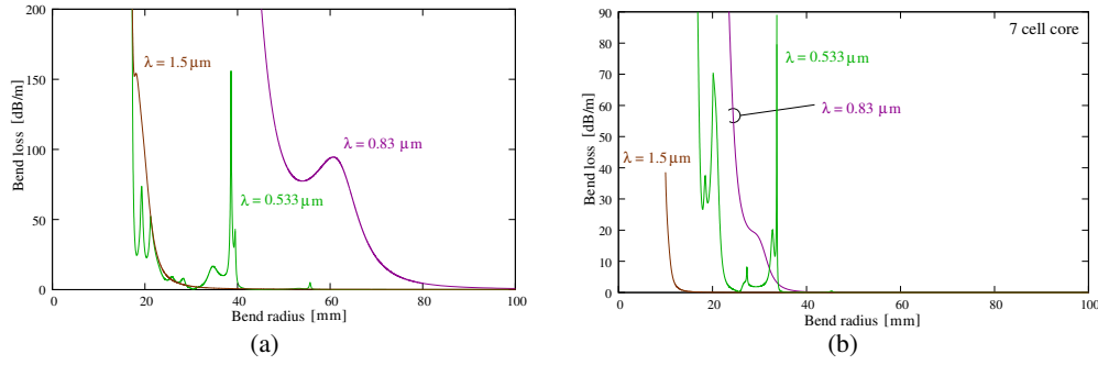
Fig. 12. Comparison of bend losses as a function of bend radius for the mid-gap wavelength of 1st, 2nd and 3rd PBGs for the structures with (a) 1 cell core and 6 cladding rings, and (b) 7 cell core and 5 cladding rings (cladding region is in keeping with that of the fiber with 1 cell core and 6 cladding rings).
