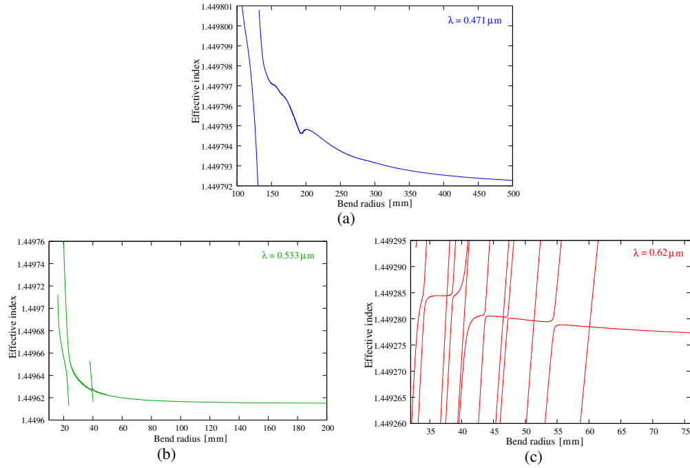
Fig. 7. Bend-radius dependence of the effective refractive indices of the modes for the fiber with 5 cladding rings for the (a) blue-edge, (b) mid-gap, and (c) red-edge wavelengths, respectively.
