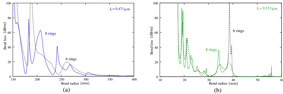
Fig. 11. Bend losses as a function of bend radius for the fiber with 8 cladding rings for (a) blue-edge and (b) mid-gap wavelengths. The bend losses for 6 cladding rings (shown in Fig. 5) are also shown with dotted curves as a reference.
