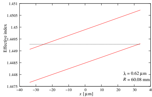
Fig. 9. Equivalent PBG edges as a function of x at the bend radius corresponding to the first appearance of the complete mode coupling (in Fig. 7(c)) for the red-edge wavelength.
