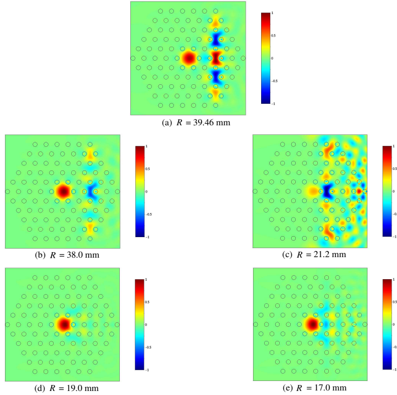
Fig. 10. x -component of the electric field distributions of the horizontally polarized modes at the loss peaks (in Fig. 8(b)) due to mode coupling between core and cladding modes for mid-gap wavelength for the 5-cladding-rings SC-PBGF with d/\Lambda = 0.4 and \Lambda = 6.75 \mu\text{m} (same as Fig. 6 except for the number of the cladding rings).
