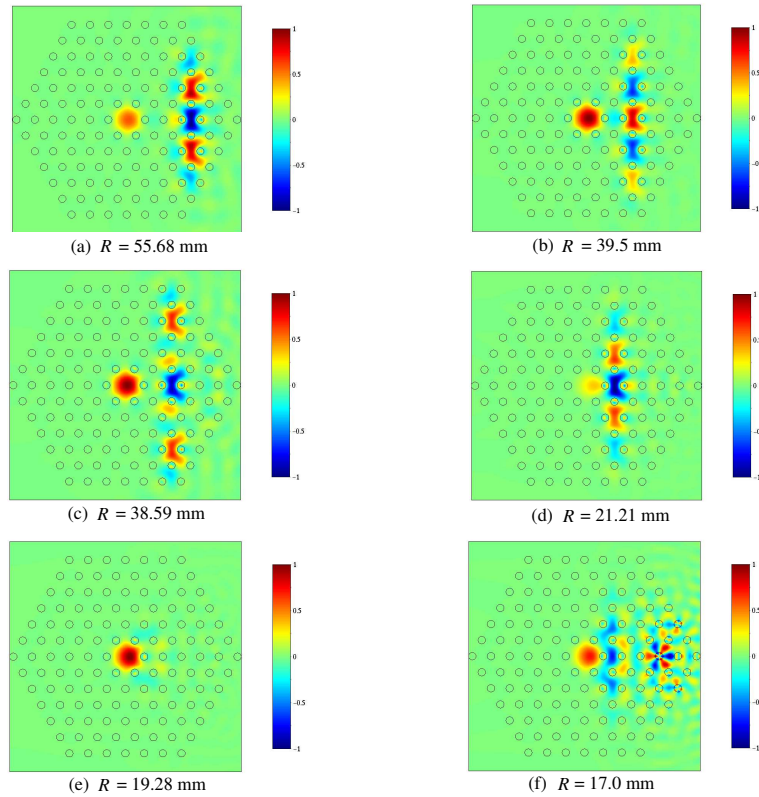
Fig. 6. x -component of the electric field distributions of the horizontally polarized modes at the loss peaks (in Fig. 5(b)) due to mode coupling between core and cladding modes for mid-gap wavelength.
