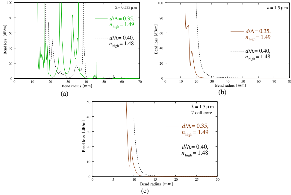
Fig. 14. Comparison of bend losses as a function of bend radius for the d/\Lambda = 0.4, n_{\text{high}} = 1.48 and d/\Lambda = 0.35, n_{\text{high}} = 1.49 at the mid-gap wavelength of (a) 3rd PBG for 1 cell-core structure, (b) 1st PBG for 1 cell-core structure, and (c) 1st PBG for 7 cell-core structure. The pitch for both structures is \Lambda = 6.75 \mu\text{m} .
