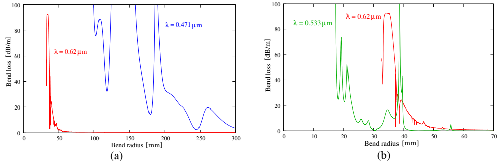
Fig. 5. Bend losses as a function of bend radius for (a) blue-edge and red-edge wavelengths, and for (b) mid-gap and red-edge wavelengths, respectively.
