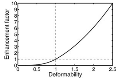
Fig. 4. Anisotropic enhancement factor \hat{E}(\mathcal{A}) as a function of the deformability \mathcal{A} according to Equation (11), for E_{\max} = 10 and E_{\min} = 0 .
