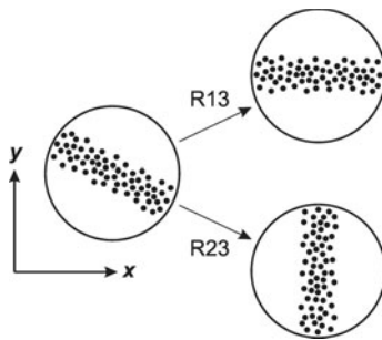
Fig. 8. Sketch of the rotation of the girdle fabrics in order to align them with the x axis (case R13) and the y axis (case R23) in the Schmidt projection.
