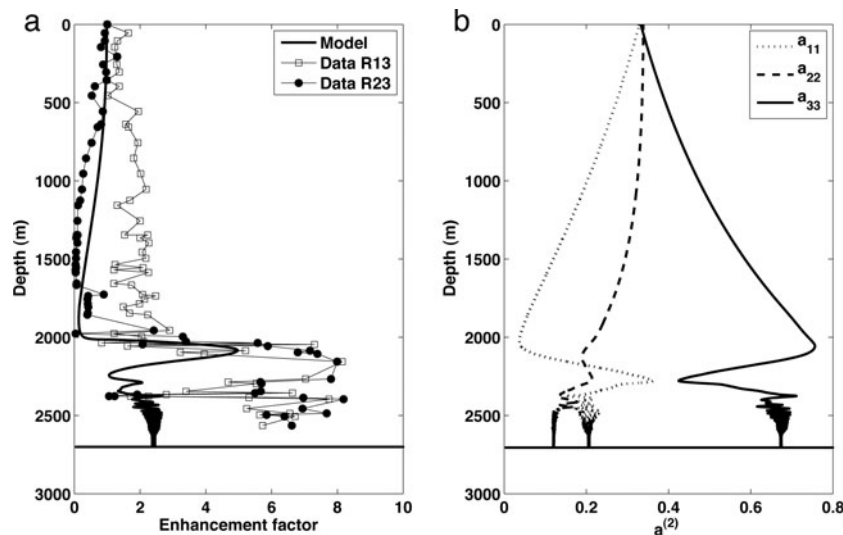
Fig. 12. Variation along the EDML ice core of (a) the enhancement factor and (b) the three non-zero components of the second-order orientation tensor a^{(2)} . 'Model' represents the solutions based on the unrestricted fabric evolution Equation (32).
