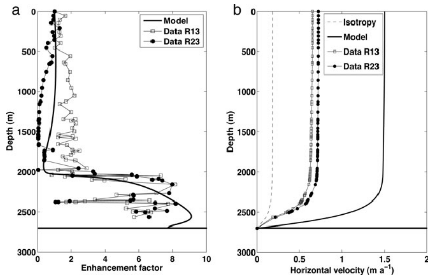
Fig. 10. Variation along the EDML ice core of (a) the enhancement factor and (b) the horizontal velocity. ‘Model’ represents the solutions based on the fabric evolution (Equation (33)) for transverse isotropy.
