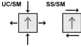
Fig. 3. Uniaxial compression on single maximum (UC/SM) and simple shear on single maximum (SS/SM) for a small sample of polycrystalline ice. Stresses are indicated by black arrows, and the single maximum fabric is represented by the dark grey arrows within the ice sample.
