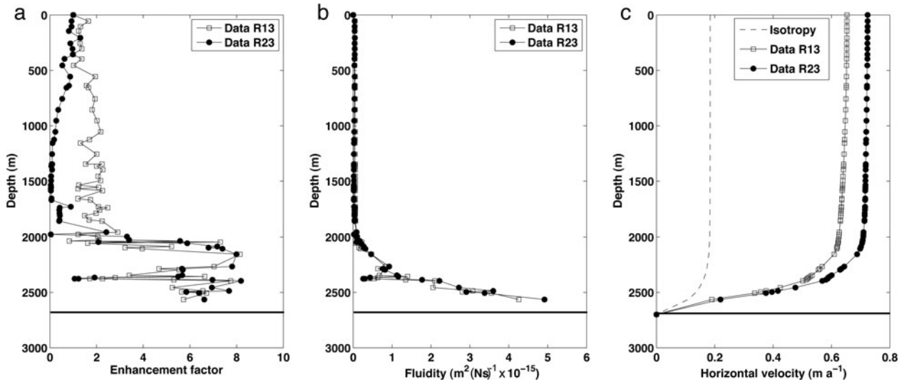
Fig. 9. Variation along the EDML ice core of (a) the enhancement factor; (b) the ice fluidity; and (c) the horizontal velocity. ‘Data R13’ and ‘Data R23’ represent the solutions obtained with the measured girdle fabrics rotated to align with the x and y direction, respectively.
