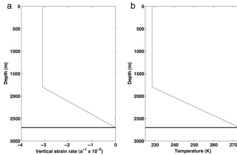
Fig. 7. Dansgaard-Johnsen distributions of (a) the vertical strain rate and (b) the temperature at the EDML site. The depth of the kinks is at two-thirds of the local ice thickness. The strain rate at the surface has been chosen such that the downward vertical velocity equals the accumulation rate and the surface and basal temperatures match the ice-core data. The bottom is indicated by the horizontal thick lines.
