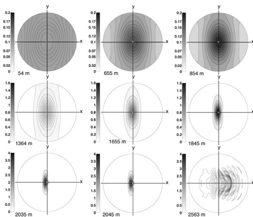
Fig. 11. Schmidt diagram representation of the EDML fabrics (ODF) at depths between 54 and 2563 m computed by Equation (32). As in Figure 5, the centres of the diagrams coincide with the core axis and the projection is on the horizontal ( x - y ) plane.
