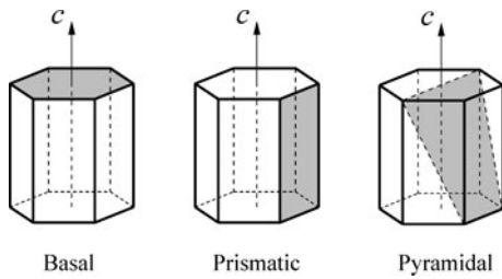
Fig. 1. Basal, prismatic and pyramidal glide planes in the hexagonal ice-I h crystal, sketched as a right hexagonal prism (Faria, 2003).
