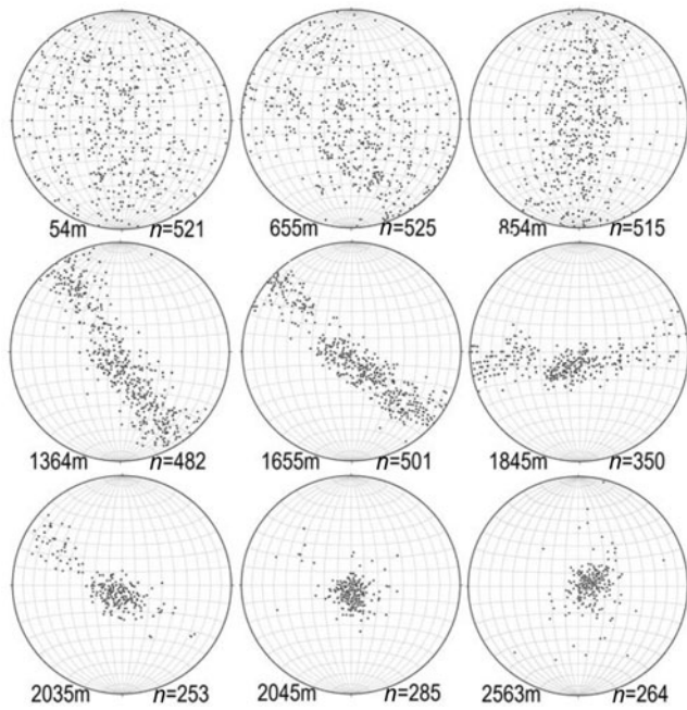
Fig. 5. Selected Schmidt diagrams for the observed fabrics of the EDML ice core between depths of 54 and 2563 m. Centres of diagrams coincide with the core axis. All examples displayed here are from vertically cut thin sections, rotated to the horizontal view. n denotes the number of grains included. Note that the orientations of the horizontal planes with respect to the ice-flow direction are unknown.
