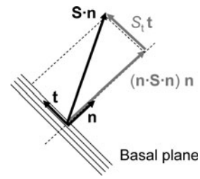
Fig. 2. Decomposition of the deviatoric stress vector ( \mathbf{S} \cdot \mathbf{n} ) into components normal ( (\mathbf{n} \cdot \mathbf{S} \cdot \mathbf{n}) \mathbf{n} ) and tangential ( S_t \mathbf{t} ) to the basal plane.
