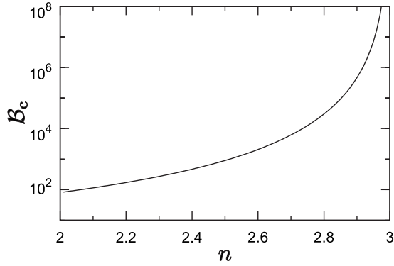
FIG. 6. The critical value B_c as a function of n . The values of B_c are plotted on logarithmic scale. We find that B_c increases with n . Eventually, in the limit n \rightarrow 3 , B_c diverges.
