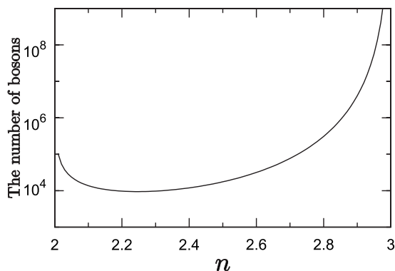
FIG. 7. The n dependence of the number of the trapped bosons in B = \tilde{U}^{-1}B_c for a given n . It has the minimal value of \sim 10^4 around n = 2.25 .
