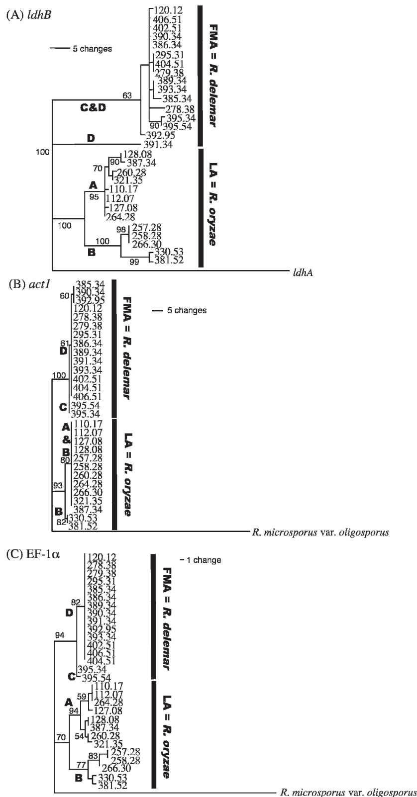
FIG. 2. Parsimonious trees based on DNA sequences of ldhB , act1 and EF-1 \alpha of R. oryzae and R. delemanii . Taxa are indicated with CBS culture numbers. Bootstrap values are shown as percentage calculated from 500 iterations. rDNA-ITS sequence types are indicated by A, B, C or D. Organic acid production groups are shown at the right of taxa. A. One of 64 most parsimonious trees based on ldhB sequence. ldhA sequence of R. oryzae NRRL 395 (accession No. AF226154, Skory 2000) was used as
