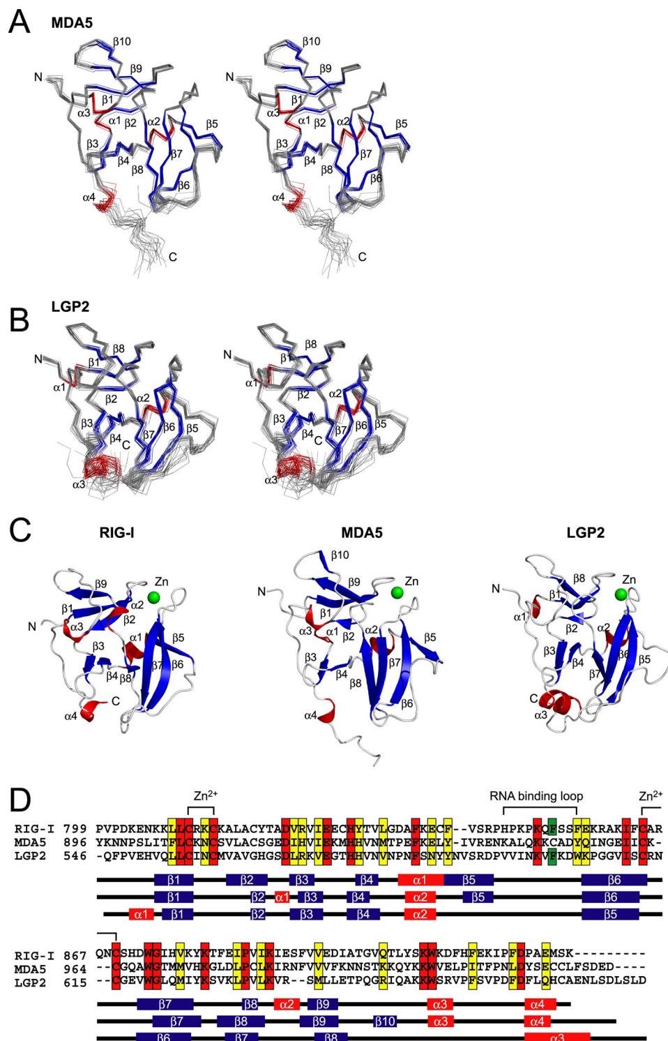
FIGURE 2. Solution structure of MDA5 CTD and LGP2 CTD. A and B, best fit superposition of the backbone atoms of 20 NMR-derived MDA5 CTD (A) and LGP2 CTD (B). Structures are shown in stereo. \beta -Strands and \alpha -helices are shown in blue and red, respectively. C, ribbon diagrams of the structure of RIG-I CTD, MDA5 CTD, and LGP2 CTD (left to right). Secondary structure elements are labeled. The figure was prepared using PyMOL. D, sequence alignment of human RIG-I, MDA5, and LGP2 CTDs. ClustalX was used to align the sequences. The secondary structure elements of each CTD are indicated below the alignment. The amino acids in red and yellow indicate conserved (red) and type-conserved (yellow) residues with the \text{Zn}^{2+} binding Cys-X-X-Cys motifs and RNA binding loop. The Phe residues conserved in RIG-I and LGP2 in the RNA binding loop are colored green.
