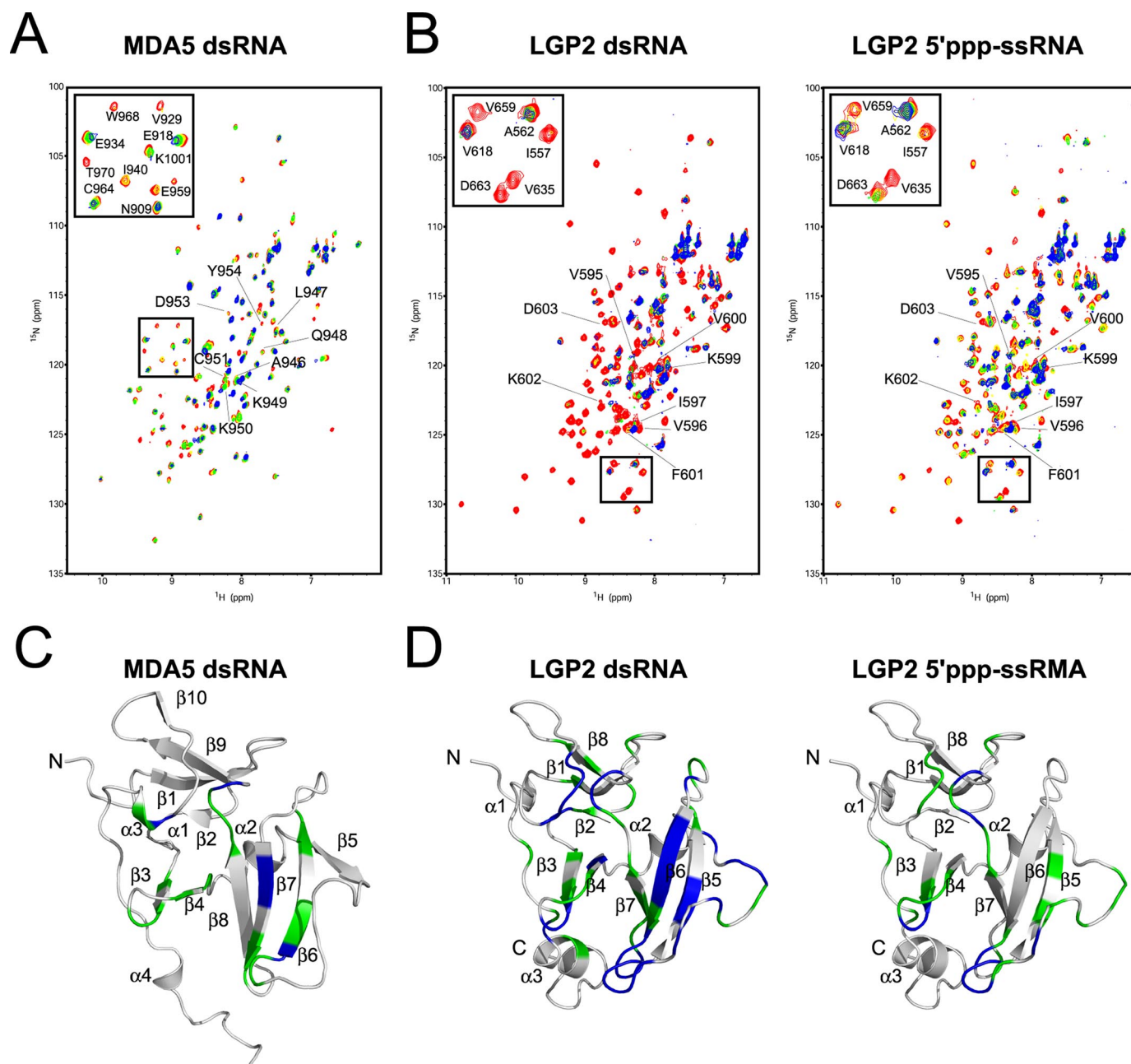
FIGURE 3. NMR titration results for MDA5 CTD and LGP2 CTD. A, NMR titration of MDA5 CTD with dsRNA. An overlay of ^1\text{H} - ^{15}\text{N} HSQC spectra are shown in red, yellow, green, and blue at 0, 0.25, 0.5, and 1.0 equivalents (molar ratio of dsRNA to proteins), respectively, where the residues in the RNA binding loop are labeled. The inset shows the excerpt of the enclosed region of the spectrum with assignment. B, NMR titration of LGP2 CTD with dsRNA (left panel) and 5' ppp-ssRNA (right panel). The figures are prepared in the same manner as in A. C, mapping of the residues of MDA5 CTD affected by the addition of dsRNA on the ribbon diagram. The residues whose peaks disappeared on addition of 0.25 and 0.5 equivalent molar ratios of dsRNA to CTD are colored blue and green, respectively. D, mapping of the residues of LGP2 CTD affected by the addition of dsRNA and 5' ppp-ssRNA (left and right panels) on the ribbon diagram, colors are the same as in C. The orientations are the same as in Fig. 2, A and B.
