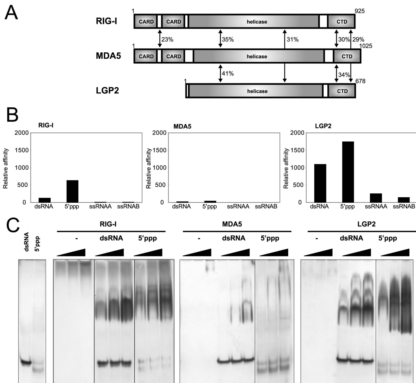
FIGURE 1. Functional analysis of RLR CTDs. A, domain structures of RIG-I, MDA5, and LGP2. Sequence identities of each domain among the RLRs are indicated. B, RNA-binding activity of RLR CTDs determined by SPR. GST-RIG-I CTD, GST-MDA5 CTD, and GST-LGP2 CTD were captured by the anti-GST antibody immobilized onto the sensor chip, then dsRNA, 5'ppp-ssRNA, and two ssRNAs (ssRNA and ssRNAB) were injected. Each resonance unit of RNA bound to a GST fused protein are standardized by molecular weight of the RNAs, then normalized by the resonance unit and molecular weight of the captured GST-fused protein. Normalized data are summarized and shown as bar graphs. RNAs bound to RIG-I, MDA5, and LGP2 are indicated from left to right in the panels. C, RNA-binding activity of RLR CTDs determined by EMSA. CTDs without the GST tag were prepared and subjected to EMSA. Increasing amounts of CTD (10, 20, and 40 pm) were reacted with the indicated probe and analyzed by native PAGE. The gels were silver-stained to visualize protein and RNA probe. —, no RNA; dsRNA, 25/25c probe; 5'ppp: 5'pppGG25 probe.
