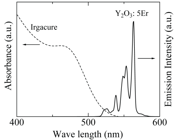
Fig.7 UC emission spectrum from \text{Er}^{3+} containing \text{Y}_2\text{O}_3 and the spectrum of the Irgacure.
