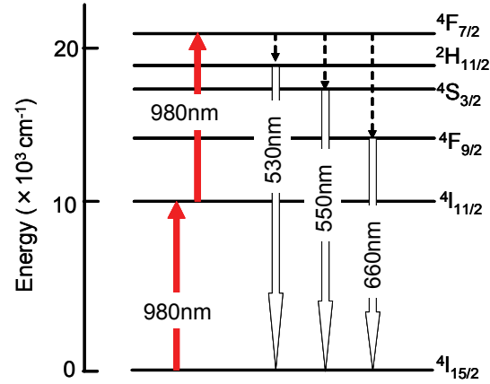
Fig.6 Energy diagram of \text{Er}^{3+} and UC emission process.
