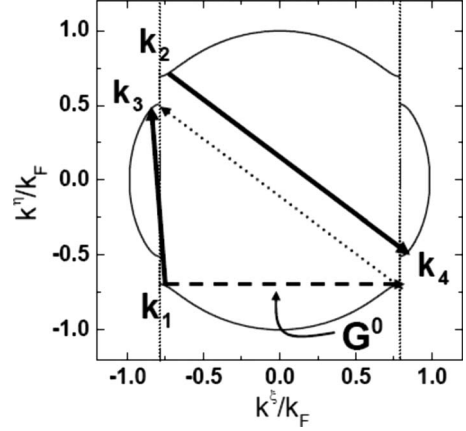
FIG. 3. Schematic illustration of first-order umklapp scattering process from between two-electron states (\mathbf{k}_1, \mathbf{k}_2) and (\mathbf{k}_3, \mathbf{k}_4) . Gaps open at k_x/k_F = \pm 0.79 , whose positions are determined by E_F and a . Here, as an example, we set E_F/U_0 = 3.13 and k_F a = 1.32 .
