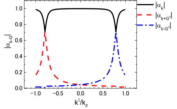
FIG. 6. (Color online) Profile of expansion coefficients |\alpha_k| as a function of k^\xi ; see Eq. (8) for its definition. The magnitude of |\alpha_{k \pm G^0}| is comparable to that of |\alpha_k| near k^\xi/k_F = \mp 0.79 , respectively, at which gaps open as shown Fig. 3.
