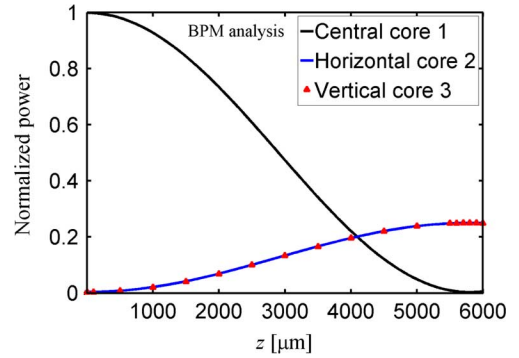
Fig. 6. Normalized power propagation in the multicore PCF power splitter ( d/\Lambda = 0.45 , d'/\Lambda = 0.23 , and \Lambda = 2.64 \text{ mm} ) at 1550 \text{ nm} wavelength calculated by the BPM simulation. It can be seen that a complete power transfer occurs at a distance of 5.8 \text{ mm} .
