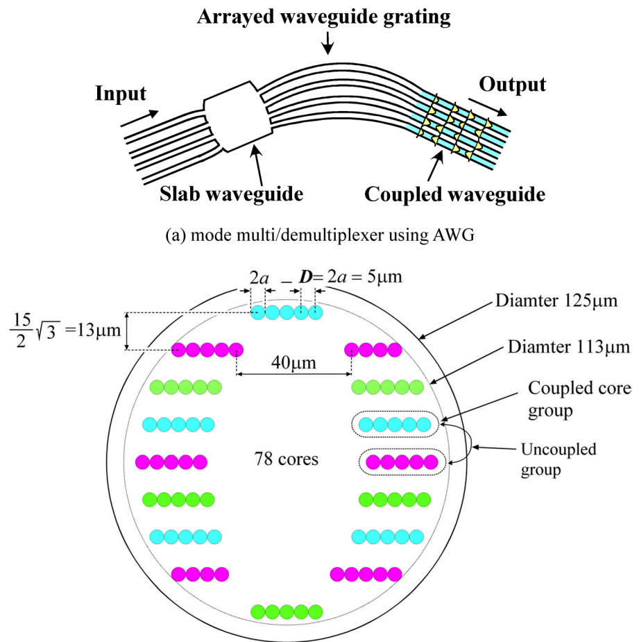
(b) hybrid configuration of coupled homogeneous multi-core and uncoupled heterogeneous multi-core fibers
