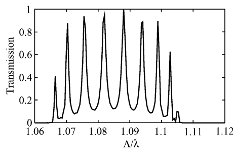
Fig. 2. Transmission characteristics for a type-1 tapered structure.
