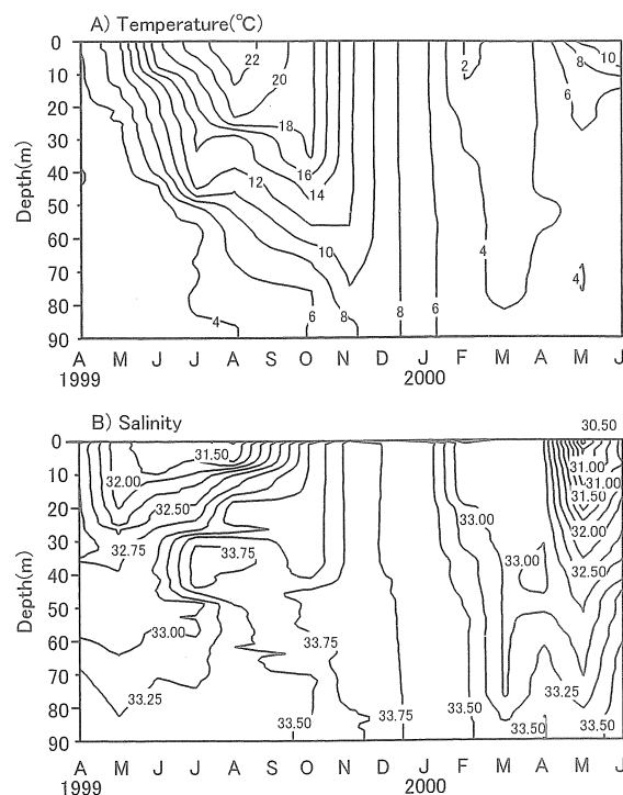
Figure 2. Seasonal changes in vertical distributions of water temperature (A) and salinity (B) at Station 30 from April 1999 to June 2000.
