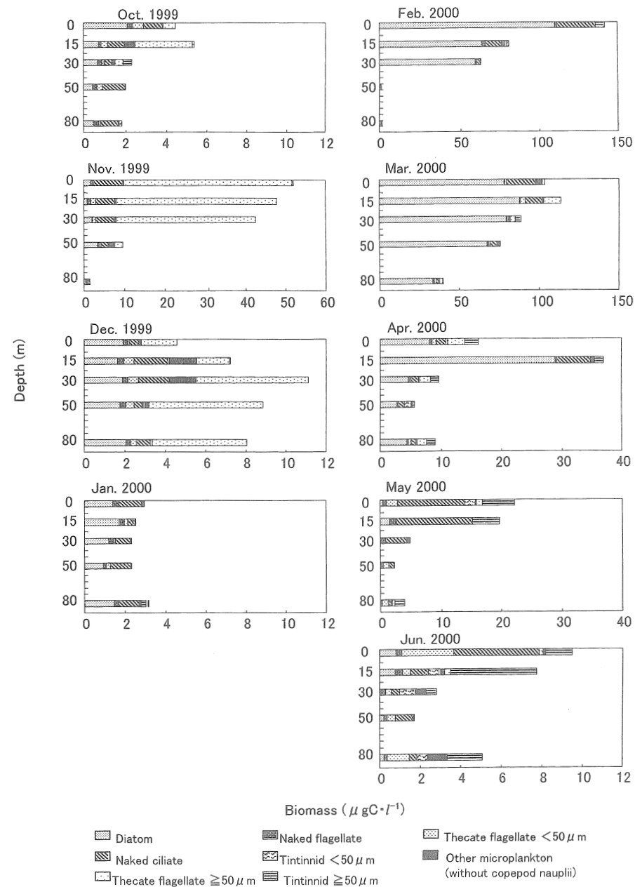
Figure 4. Vertical distributions of microplankton biomass (10–200 \mu\text{m} ) at Station 30 from October 1999 to June 2000.
