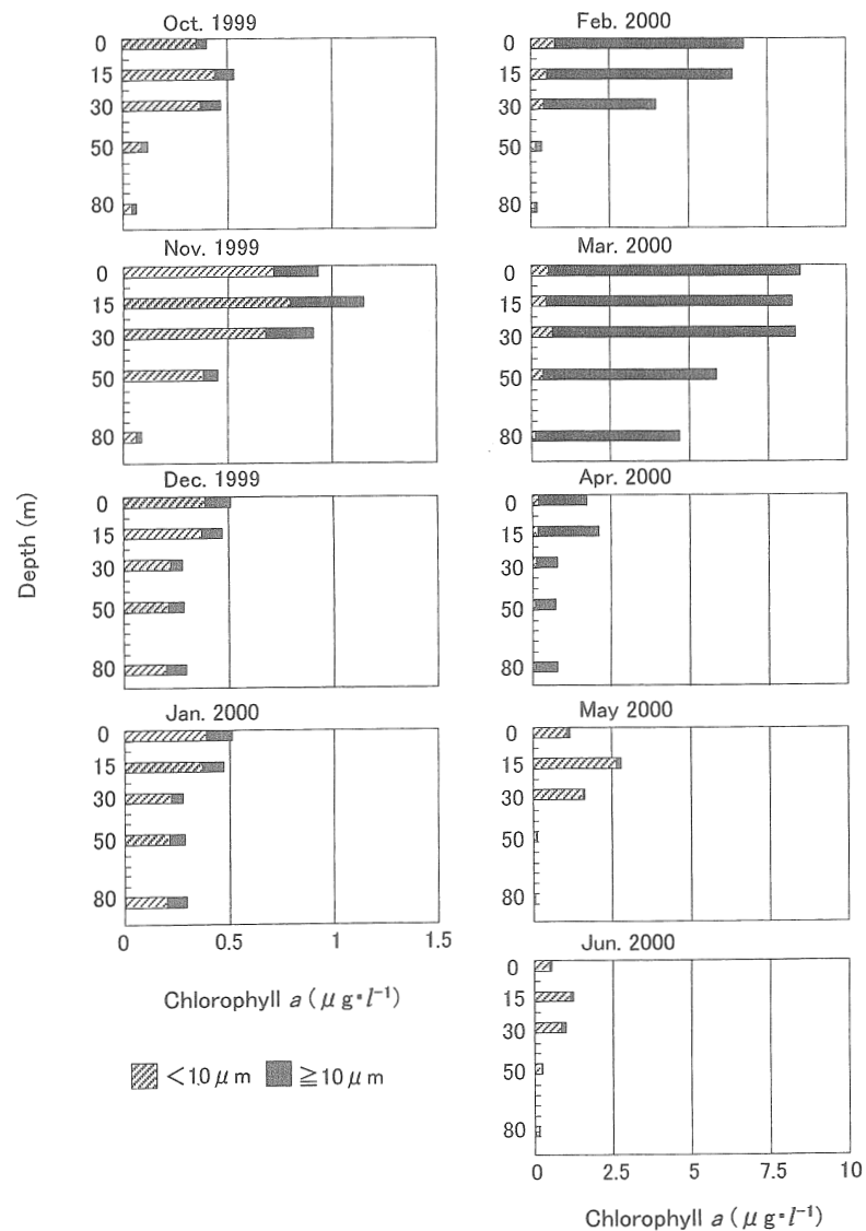
Figure 3. Vertical distributions of chlorophyll a concentration at Station 30 from October 1999 to June 2000.
