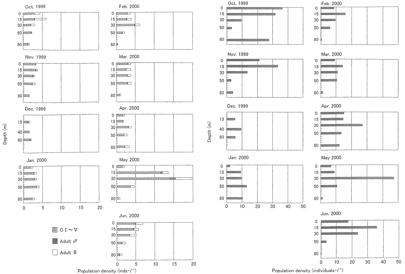
Figure 7. Vertical distributions of Oithona nauplii (right) and copepodids (left) at Station 30 from October 1999 to June 2000. Samples were collected with Van-Dorn bottles at three depths (15, 40, 60 m) in December 1999 and at five depths (0, 15, 30, 50, 80 m) in other months.
