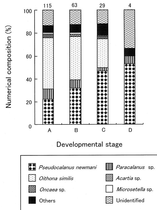
Figure 4. Numerical compositions of copepod nauplii in digestive tracts of C. pinetorum larvae by developmental stage. The numeral above each bar shows the number of nauplii identified.
