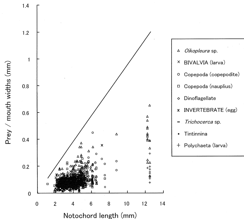
Figure 3. Prey size distribution of food items in digestive tracts of C. pinetorum larvae in Funka Bay during 10–20 August 2001. The solid line shows the regression line between notochord length (NL) and mouth width (MW) of larvae ( MW=0.0952NL , N=329 , r^2=0.72 , P<0.001 ).
