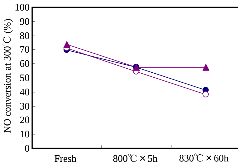
Fig. 3 The NO oxidation activity of different noble metal catalysts, Pt(0.77), Pt(0.94), and Pt(0.77)Pd(0.30), fresh and heat-treated at 800°C and 830°C. Catalysts: (●) Pt(0.77), (○) Pt(0.94), (▲) Pt(0.77)Pd(0.30).
