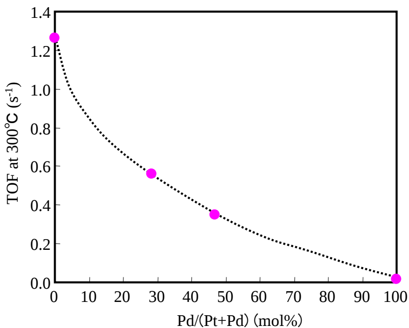
Fig. 11 Change of NO oxidation TOF with Pd content for Pd-modified Pt catalysts heat treated in air at 830°C for 60 h
