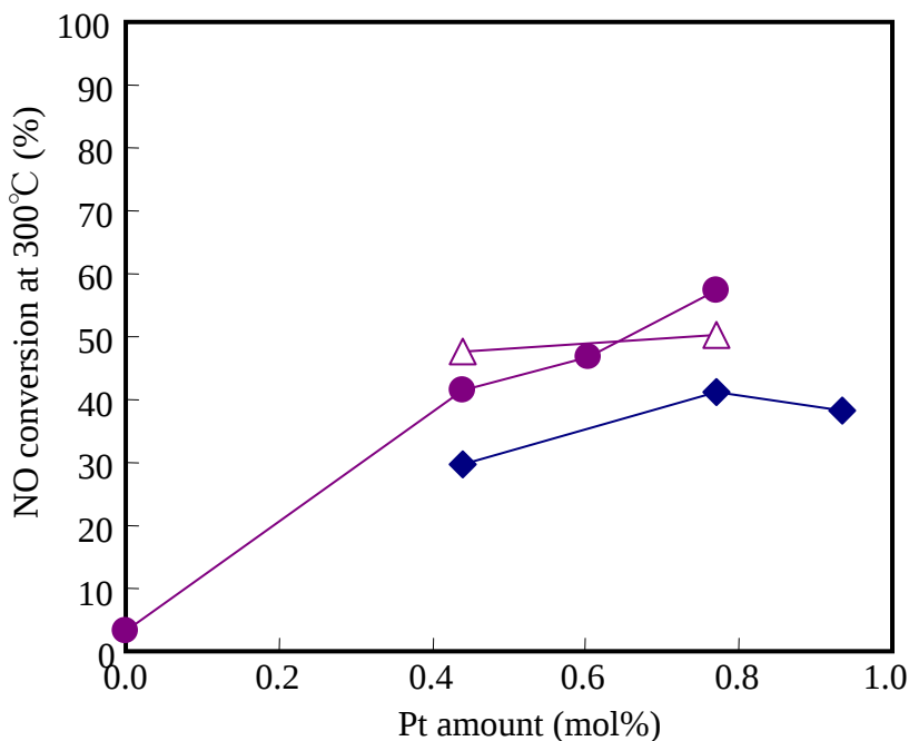
Fig. 2 The NO oxidation activity of various noble metal catalysts after heat treatment in air at 830°C for 60 h. Pd content: ♦ none; ● 0.30 mol%; △ 0.68 mol%
