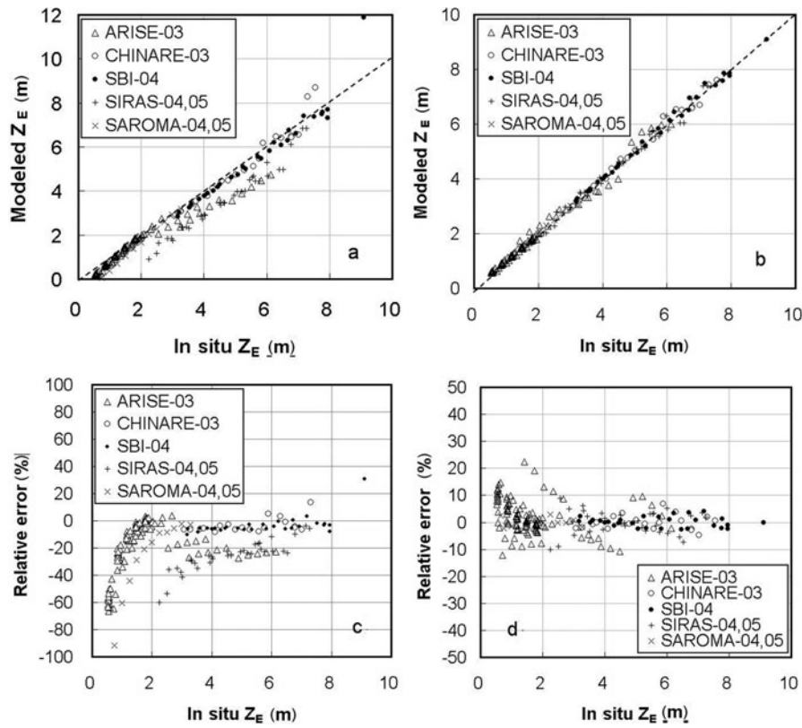
Fig. 5. Relationships between the in situ measured Z_E and Z_E calculated with (a) a simple three-layer model of snow ( \sigma_s = 0 \text{ mS m}^{-1} ), ice ( \sigma_i = 52 \text{ mS m}^{-1} ) and sea water ( \sigma_w = 2482 \text{ mS m}^{-1} ), and (b) the standardized model. Relative errors are shown between the in situ measured Z_E and the Z_E calculated using (c) a simple three-layer model and (d) the standardized model.
