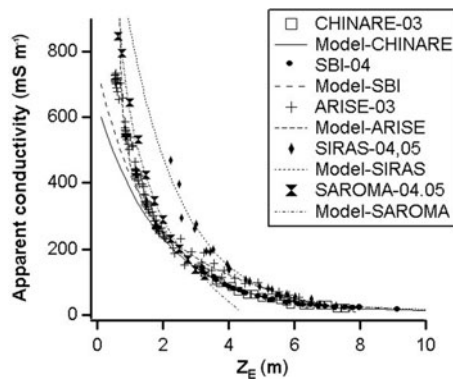
Fig. 2. Derived \sigma_a - Z_E relationships from calibrations made by changing the EM instrument height in the Chukchi Sea, off East Antarctica, in the Sea of Okhotsk and in Saroma-ko. The curves are exponential fits to the data points.
