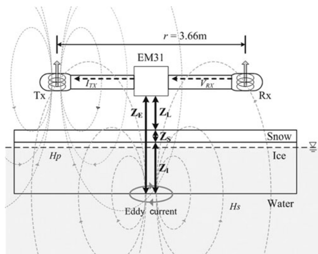
Fig. 1. Schematic of measurement of sea-ice thickness with the EM31/ICE. The distances Z_E , Z_L , Z_S and Z_I are respectively from instrument to ice bottom, from instrument to snow surface, snow depth, and ice thickness.
