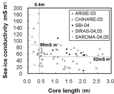
Fig. 4. Relationship between the bulk sea-ice conductivity and ice-core length.
