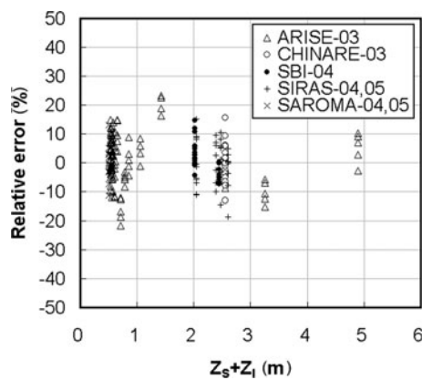
Fig. 6. Relative errors between the modeled Z_s + Z_i calculated using the standardized model and the in situ measured Z_s + Z_i .
