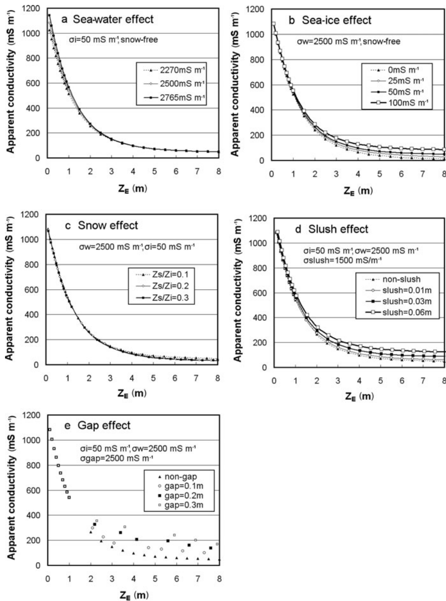
Fig. 3. Effects on the \sigma_a - Z_E relationships due to changes in (a) sea-water conductivity, (b) sea ice conductivity, (c) snow depth, (d) depth of saline wet snow 'slush' layer on the ice, and (e) sea-water-filled gaps between deformed ice floes. The floes have a maximum thickness of 1 m. All calculations use Z_L = 0 m and \sigma_s = 0 mS m -1 .
