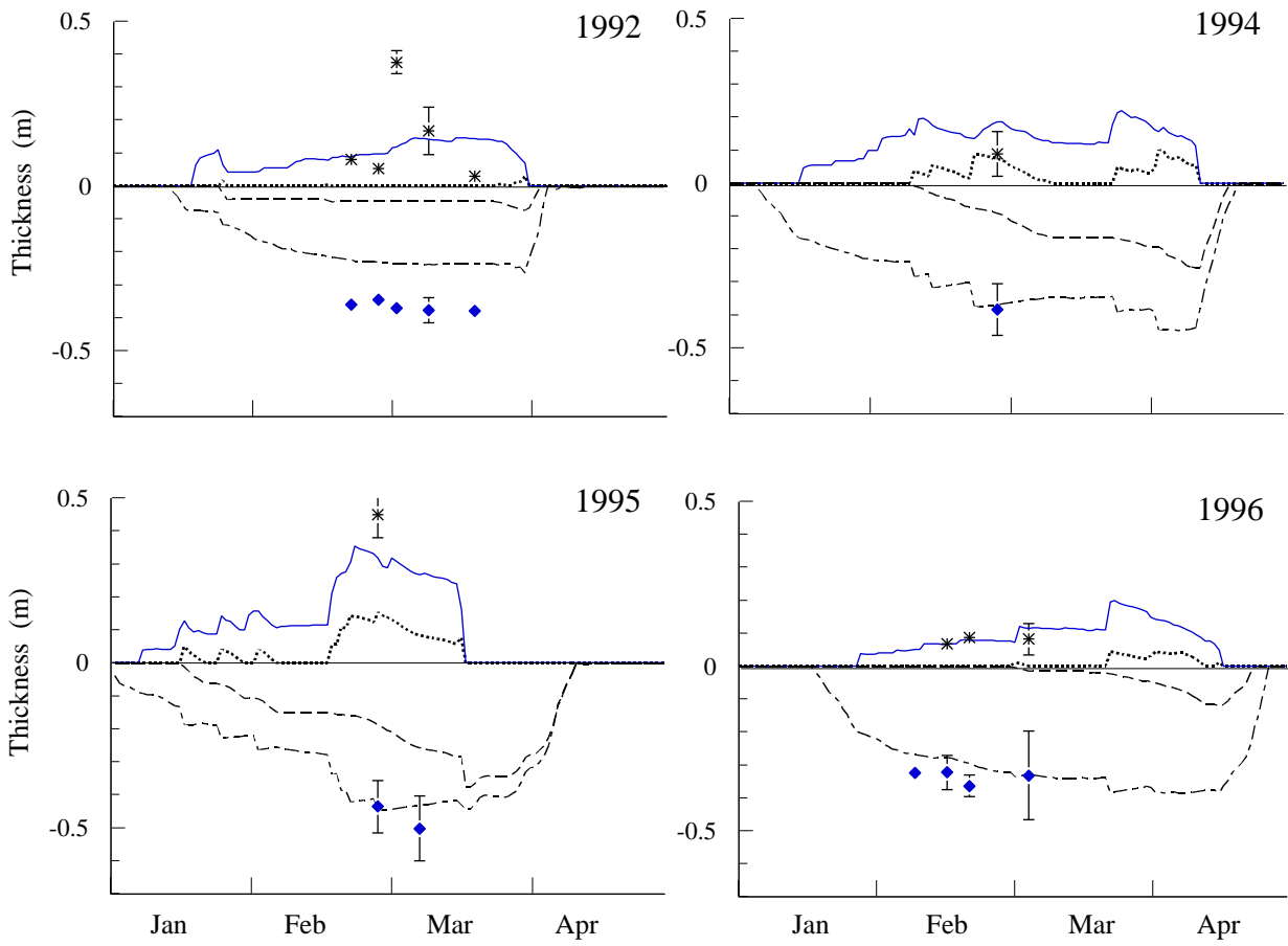
Fig.3 The model outcome of the thicknesses of congelation ice, snow-ice and snow for Saroma-ko Lagoon, 1992 and 1994-1996, shown together with observations.
